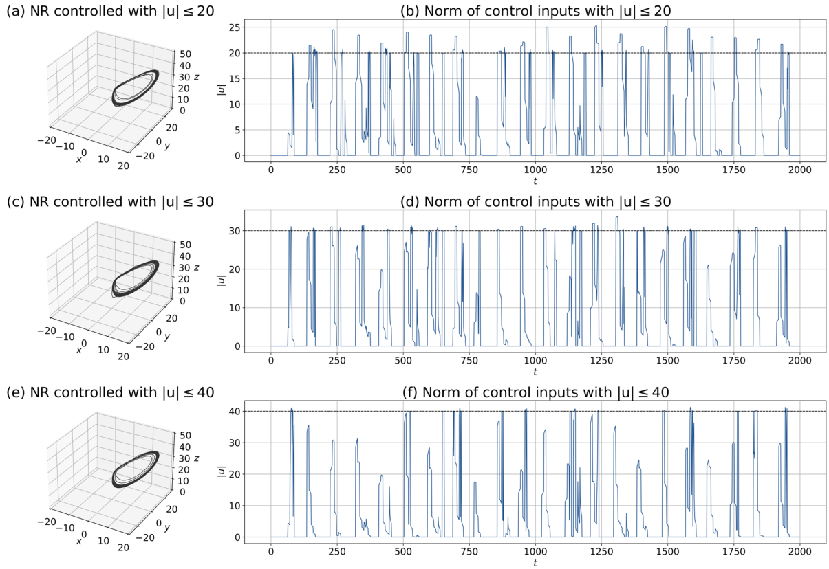
Figure 8: The MPC experiments with inequality constraints for control inputs \|\mathbf{u}^*\| \leq U : (a, b) U = 20 , (c, d) U = 30 , and (e, f) U = 40 . (a, c, e) show the NRs, and (b, d, f) show the L^2 norm of control inputs. The dashed lines in (b, d, f) show the prescribed upper limits of the control inputs (i.e., U = 20, 30 and 40 ). Each starting point is identical to Fig. 3 (i.e., the 24th step of two-million-step DA cycles).
