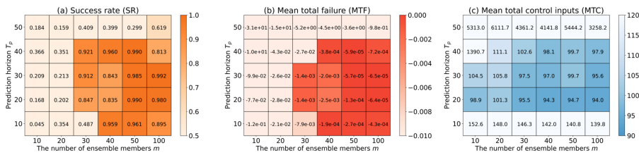
295 Figure 6: Sensitivity to the prediction horizon T_p and the ensemble size m with three evaluation indicators: (a) success rate (SR), (b) mean total failure (MTF), and (c) mean total control inputs (MTC). Darker colors in (a), (b) and (c) indicate better controllability.
