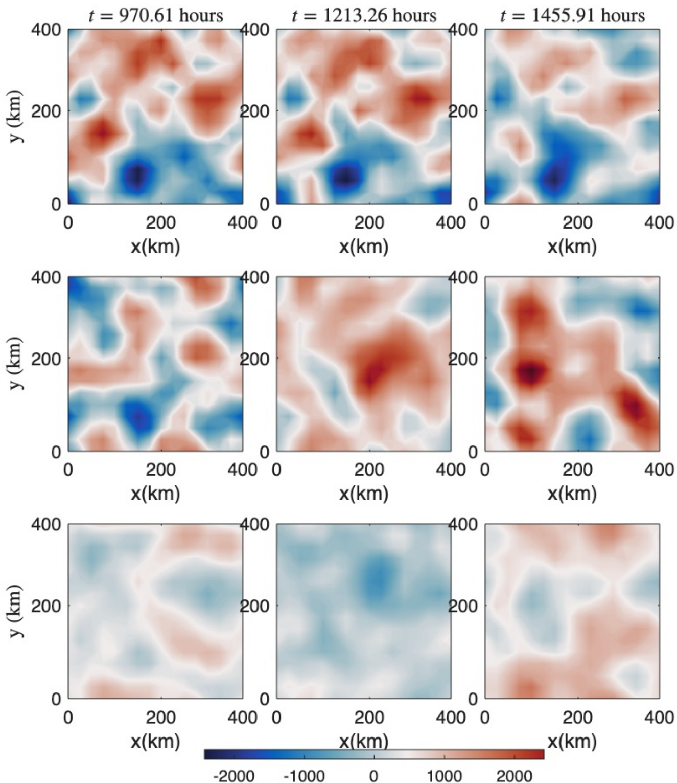
Figure 7. Recovered upper-layer ocean streamfunction: comparison among the truth (top panel), the posterior mean (middle panel) and the posterior mean (bottom panel) at different time instances.
