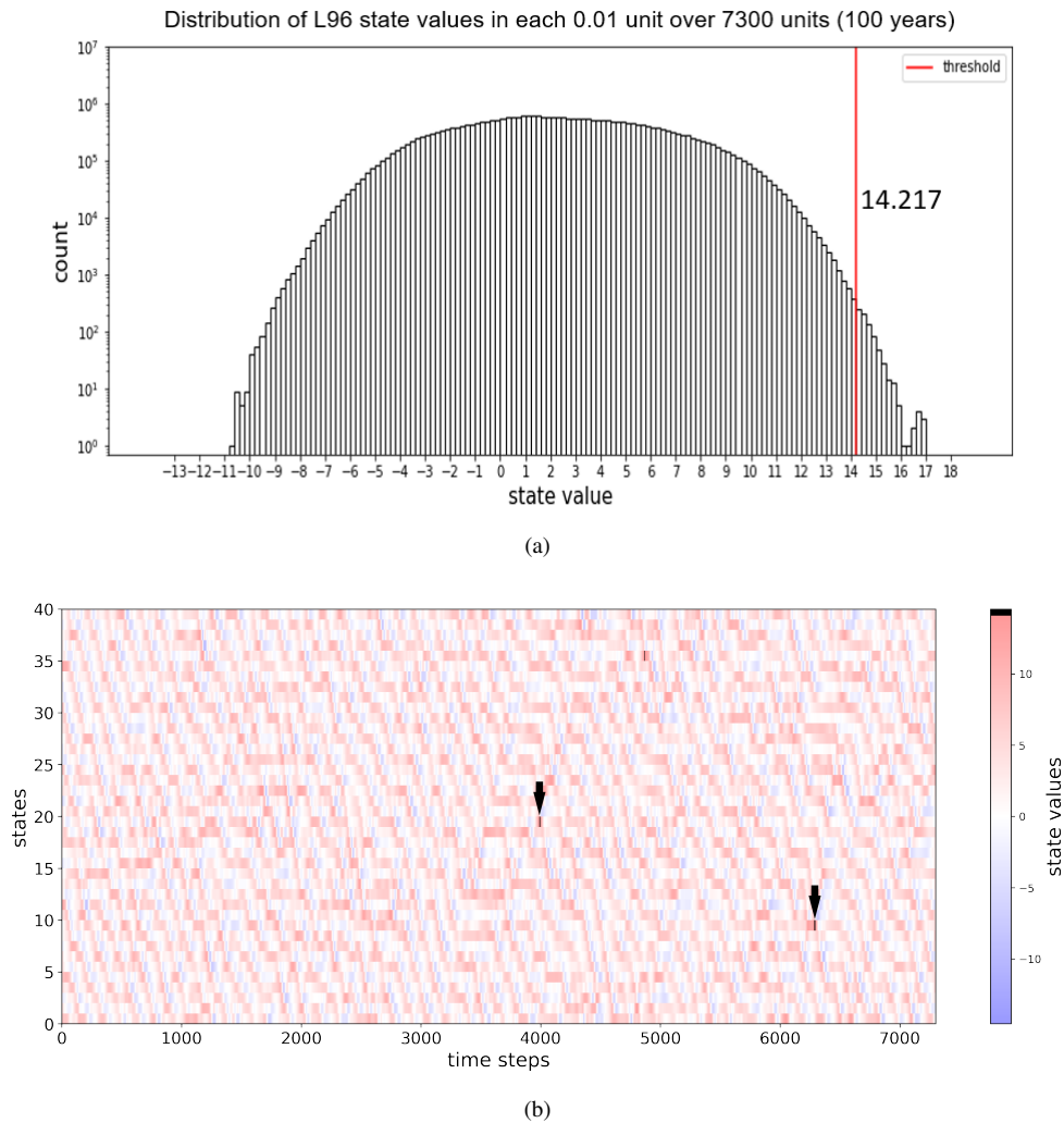
Figure 2. (a) The distribution of the state values of Lorenz-96 recorded every 0.01 unit of time for 7300 units, (b) The values of all states over a randomly chosen year. The extreme values are colored in black and indicated by arrows.
