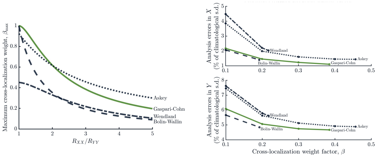
Figure B3. Left: Maximum cross-localization weight factor as a function of R_{XX}/R_{YY} . Right: Average analysis errors are shown on the y-axis for different multivariate functions. The top (bottom) plot shows analysis errors for the X ( Y ) process. For all functions, as the cross-localization weight factor increases, the analysis errors decrease. Analysis errors are calculated as RMS deviations from the “truth” and are scaled by the climatological standard deviation of the associated process.
