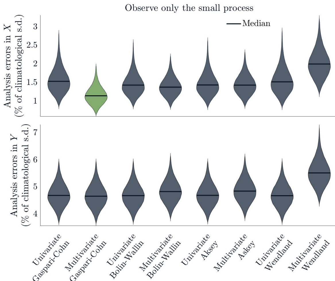
Figure 3. Violin plots show the distribution of analysis errors for the X and Y process with different localization functions (Hoffmann, 2015). Analysis errors are calculated as RMS deviations from the “truth” and are scaled by the climatological standard deviation of the associated process. All four univariate localization functions perform similarly, while there is a greater range in performance for the multivariate versions of these functions. Multivariate Gaspari-Cohn shows improvement over its univariate counterparts. Univariate and multivariate Bolin-Wallin and Aksey functions appear to perform similarly. For Wendland, the multivariate function performs significantly worse than the univariate function.
