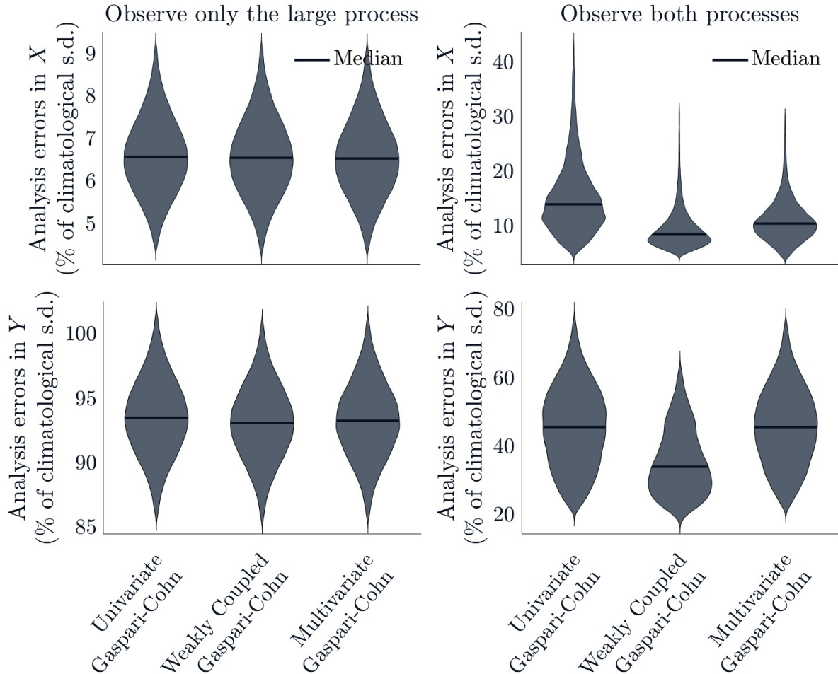
Figure 4. Violin plots show the distribution of analysis errors for all versions of the Gaspari-Cohn localization function (Hoffmann, 2015). Analysis errors are calculated as RMS deviations from the “truth” and are scaled by the climatological standard deviation of the associated process. Left: results from the experiment where we observe only the “large” process. All functions perform similarly. Right: results from the experiment where we observe both processes. The weakly coupled localization functions appear to lead to the best performance, but are highly unstable.
