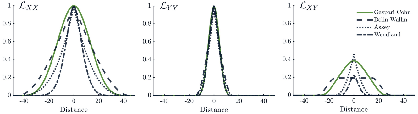
Figure 1. Four multivariate localization functions are shown in three panels. The first panel shows the function \mathcal{L}_{XX} used to localize the “large” process, X . The second panel shows the function \mathcal{L}_{YY} used to localize the “small” process, Y . The third panel shows the cross-localization function \mathcal{L}_{XY} . In each panel, the color of the line shows the different multivariate functions: Gaspari-Cohn (green, solid), Bolin-Wallin (dark, dashed), Askey (dark, dotted), and Wendland (dark, dash-dot). In the case of univariate localization, the functions in the middle panel are used to localize all processes. The within component localization radii are R_{YY} = 15 and R_{XX} = 45 for all functions. The cross-localization radii are R_{XY} = 30 for Gaspari-Cohn and Bolin-Wallin and R_{XY} = 15 for Askey and Wendland.
