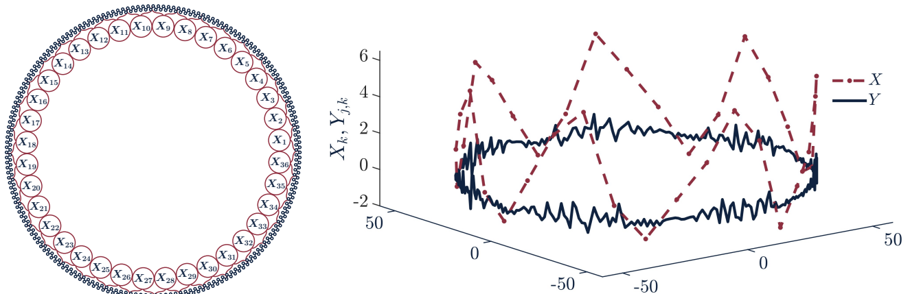
Figure 2. Left: Schematic illustrating the location of the different variables in the bivariate Lorenz 96 model, inspired by Wilks (2005). The setup has K = 36 sectors, with J = 10 “small” process variables per sector. The “large” process is shown on the inner circle and each X variable is labeled. The “small” process is shown, unlabeled, on the outer circle. Brackets show the sectors. Right: A single snapshot of the bivariate Lorenz 96 model with variables placed on a circle. The “large” process X (red, dashed) has fluctuations with amplitude about 10 times larger than the fluctuation of the “small” process Y (dark, solid).
