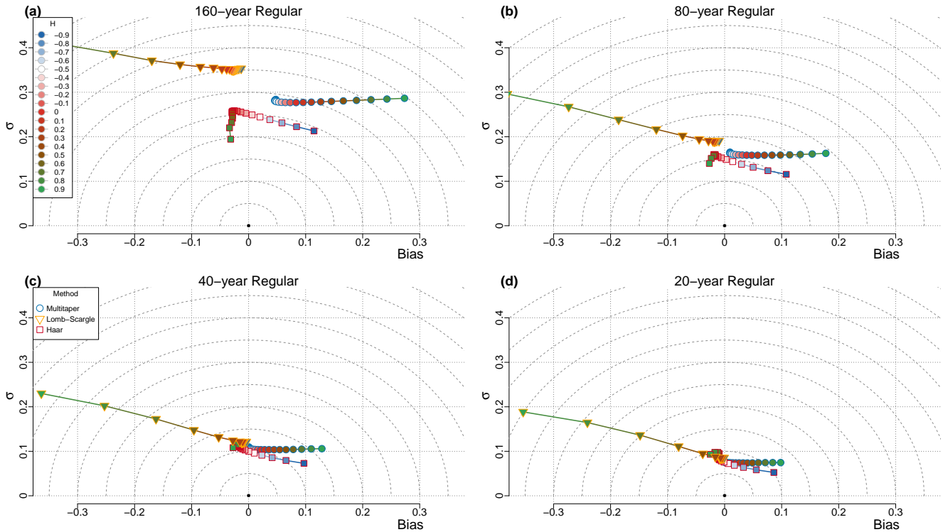
Figure 5. Resolution dependence of the estimators. The performance of the estimators is shown for regular surrogate data of different resolutions: (a) 160 years , (b) 80 years, (c) 40 years and (d) 20 years. For each case, the series spanned 5120 years, and therefore each case contains 32, 64, 128 and 256 data points, respectively.
