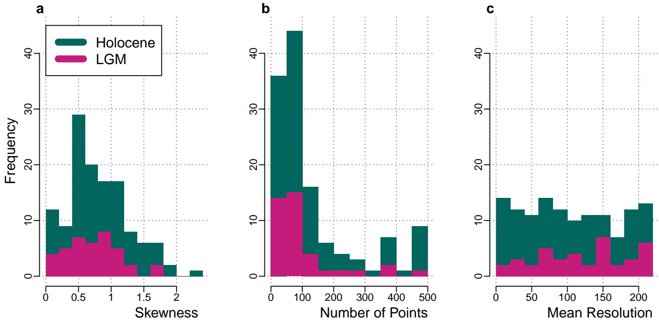
Figure 2. Sampling characteristics of the 127 paleoclimate timeseries (Rehfeld et al., 2018). The 88 Holocene series (teal) and 39 Last Glacial Maximum series (pink) are evaluated along the following characteristics: (a) the skewness \nu of the distribution of time steps, (b) the number of points, i.e. samples, and (c) the mean resolution \tau_\mu of the time steps.
