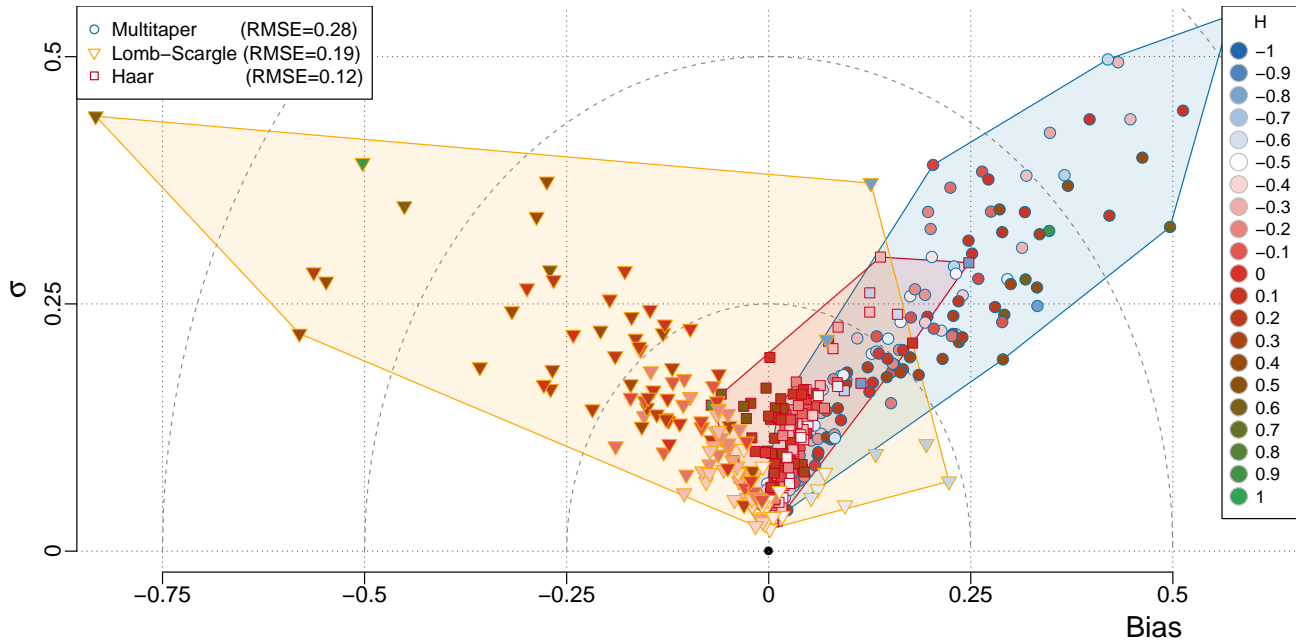
Figure 7. Bias-standard deviation diagram for the surrogate timeseries generated using timesteps from the paleoclimate database. The input H used to generate the timeseries is indicated by the colour inside the markers. The shaded polygons contain all the points for a given method (see legend for colours).
