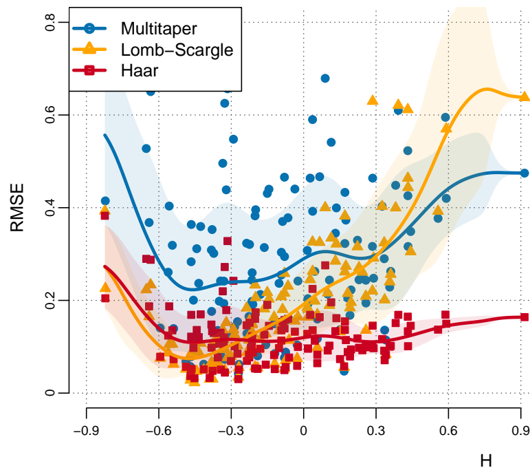
Figure 8. RMSE of the H estimates as a function of the input H for the surrogate timeseries based on the proxy database. The RMSE are given for the three estimation methods as a function of the H used to generate the surrogates. Also shown is a Gaussian smoothing of the points for each method (thick line) and the one standard deviation confidence interval (shaded).
