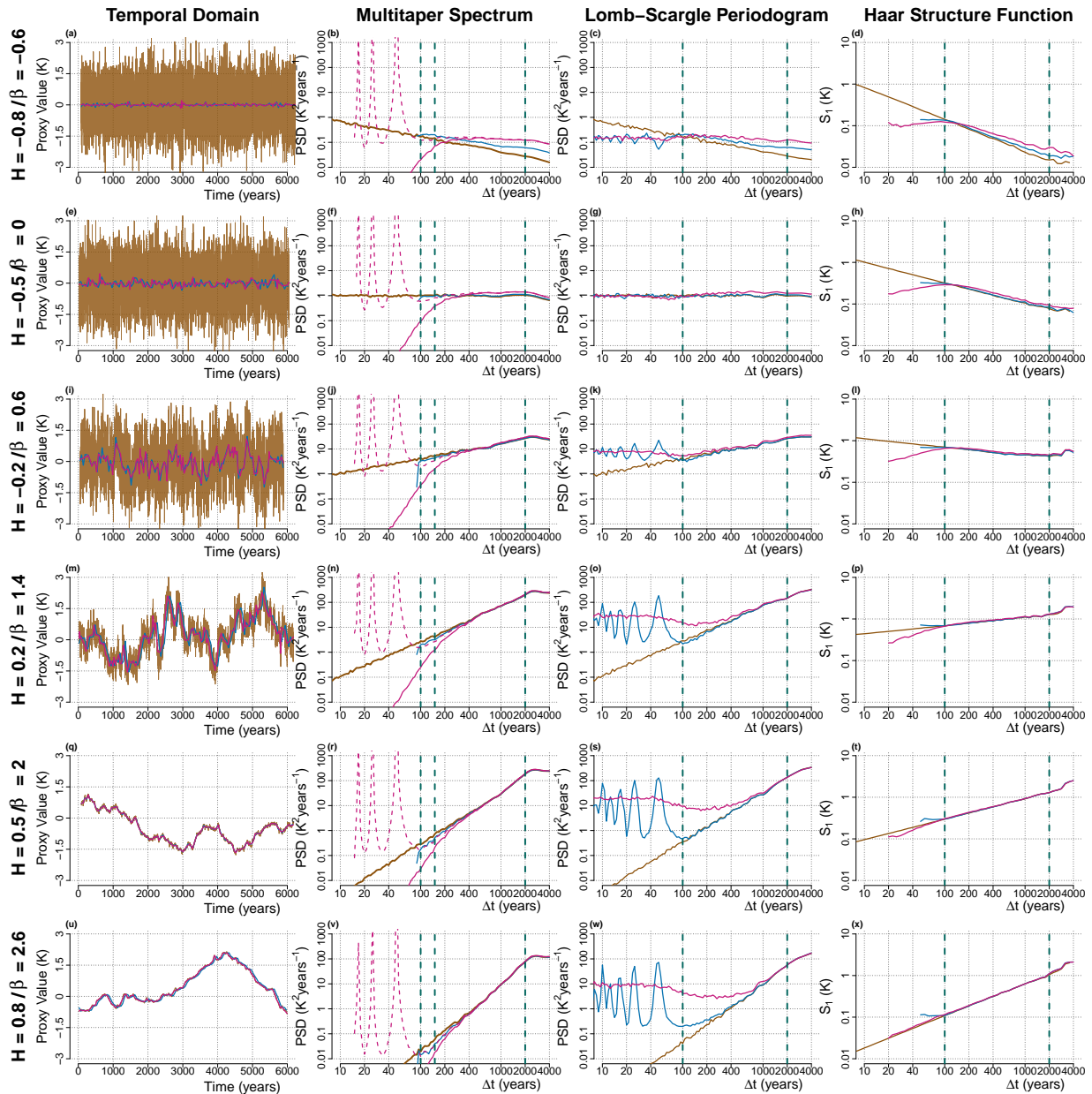
Figure 1. (a,e,i,m,q,u) Surrogate timeseries generated with a given H are shown at annual resolution (brown), degraded to a regular 50-year resolution (blue) and degraded to an irregular and random spacing drawn out of a gamma distribution with skewness \nu = 1 and mean 50 years. (b,f,j,n,r,v) Shown are the mean power spectra, estimated using the MTM, of 100 realizations of surrogate timeseries generated as in (a,e,i,m,q,u), respectively, and shown with the same colour scheme. The irregular case is also shown after dividing the power spectra by the expected \text{sinc}^4 bias due to interpolation (dashed pink). Also shown are the bounds for the fitting range considered later (vertical dashed blue): at the Nyquist frequency corresponding to 100 years, at 1.5 times the Nyquist frequency corresponding to 150 years and at one third the length of the timeseries at 2000 years. c,g,k,o,s,w Same as (b,f,j,n,r,v), respectively, but for the LSP instead of the MTM. d. Same as (b,f,j,n,r,v), respectively, but showing HSF instead of MTM power spectra.
