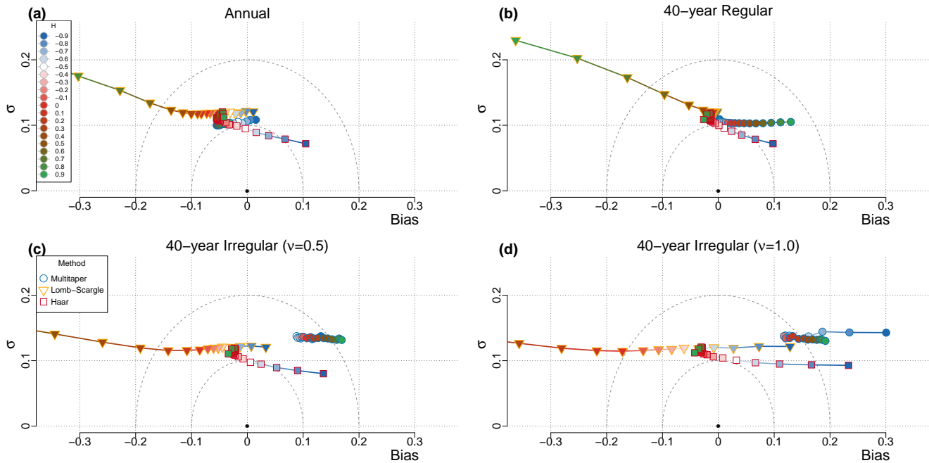
Figure 3. Bias-Standard Deviation diagram for ensembles of H estimates surrogate timeseries with input values of H \in (-1, 1) (i.e. \beta \in (-1, 3) ). Different types of data are evaluated: (a) regular “annual data”, i.e. it was directly simulated and not degraded after, (b) regular ‘surrogate data degraded at regular 40-year interval, and irregular surrogate data with timesteps drawn from a gamma distribution with (c) skewness \nu = 0.5 or (d) skewness \nu = 1 .
