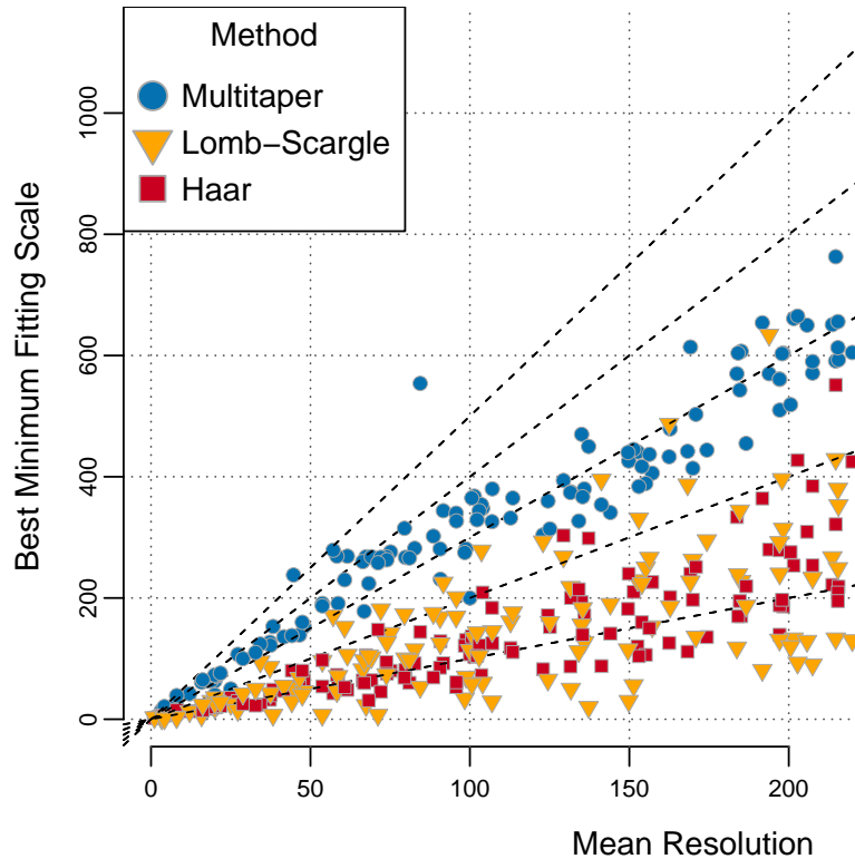
Figure 6. Best minimum fitting timescales. For each methods are shown the best minimum fitting timescales \tau_{min} (minimizing the RMSE in H ) as a function of the mean resolution \tau_{\mu} for ensembles of surrogate data generated with the same sampling scheme as the corresponding paleoclimate timeseries from the database.
