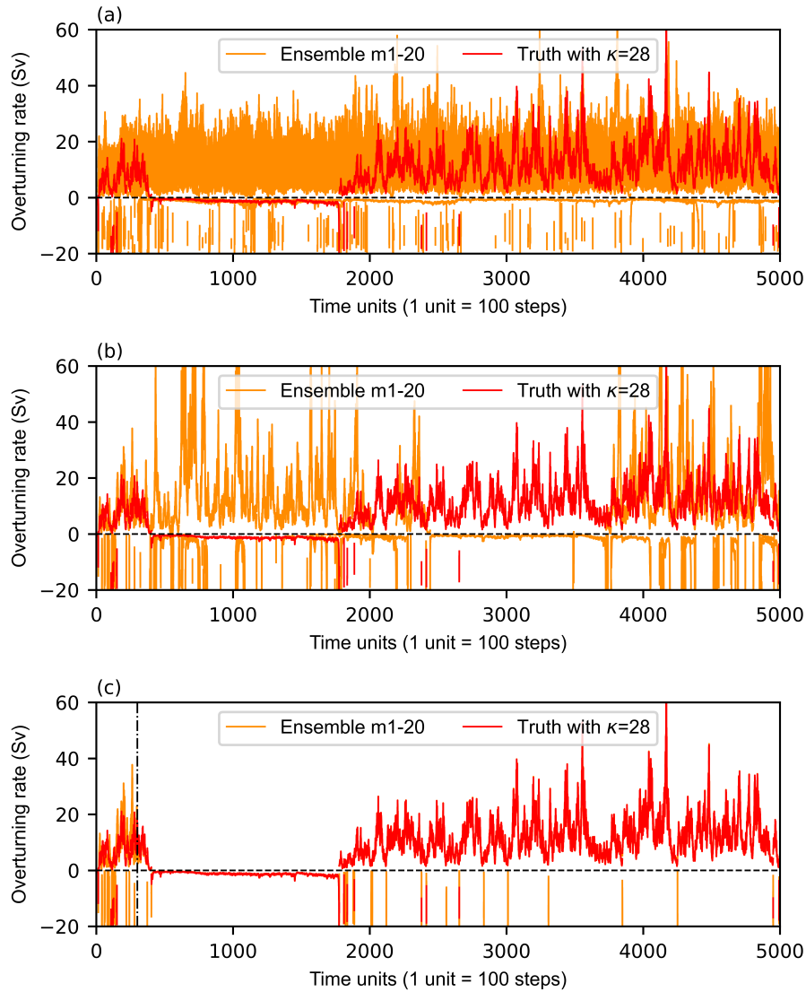
510 Figure 5. Time series of the overturning rate in the “truth” simulation with \kappa = 28 (red) and the individual ensemble members (orange) in the free model control ensemble simulations a) without data assimilation and parameter estimation, b) with data assimilation or c) with data assimilation and parameter estimation using erroneously-guessed \kappa values with a Gaussian perturbation that has a mean value of 32 and a standard deviation of 0.1. The dashed black line denoting \nu = 0 is a division line between the thermal mode equilibrium state and the haline mode equilibrium state. The dotted-dashed black line denoting 300th-unit marks the start of parameter estimation.
