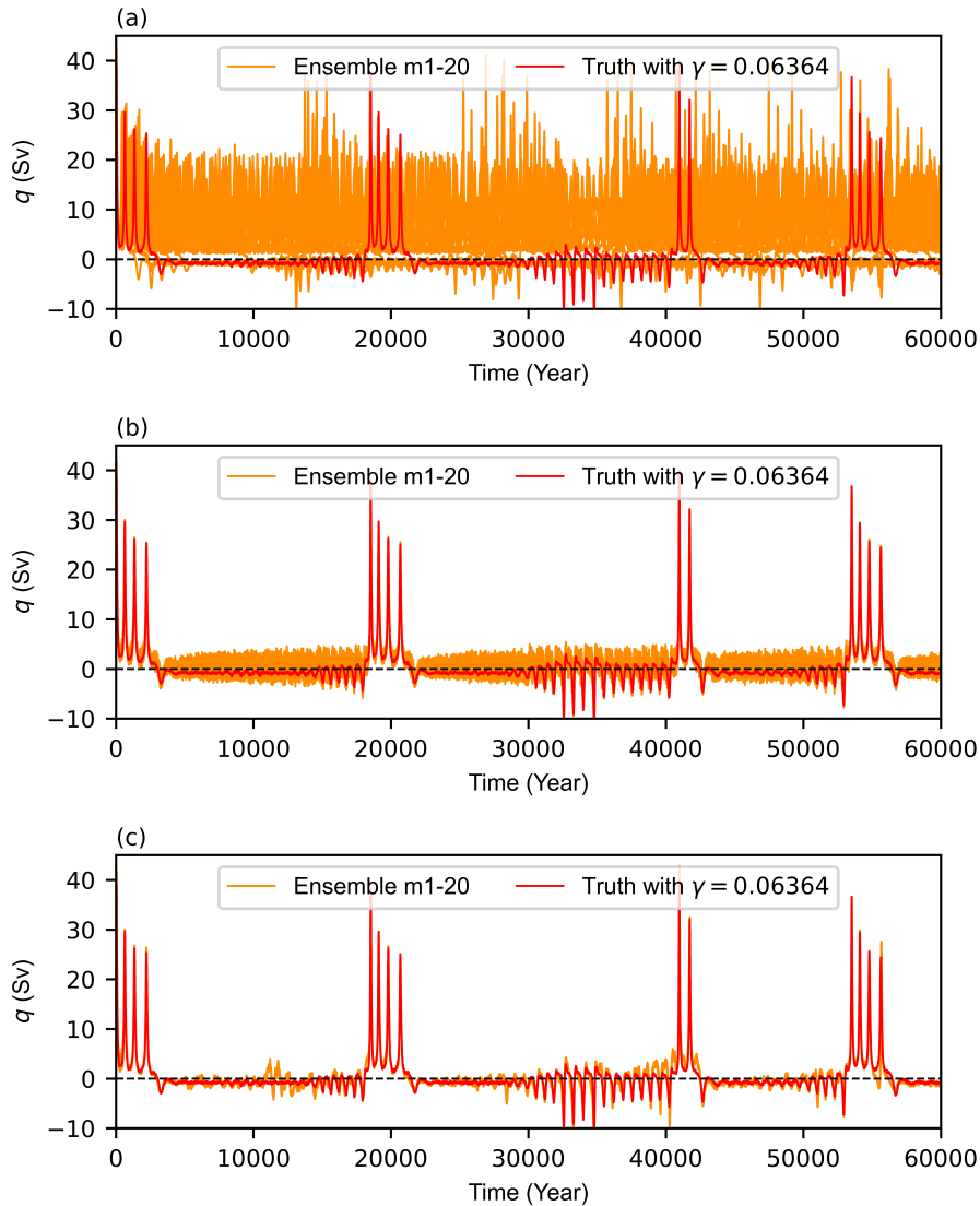
610 Figure 9. Time series of the meridional overturning circulation q in the “truth” simulation with \gamma = 0.06364 (red) and the individual ensemble members (orange) in the free model control ensemble simulations a) without data assimilation and parameter estimation, b) with data assimilation or c) with data assimilation and parameter estimation using erroneously-guessed \gamma values with a Gaussian perturbation that has a mean value of 0.070004 and a standard deviation of 10% times the standard value. The dashed black line denoting q = 0 is a division line between two equilibrium states.
