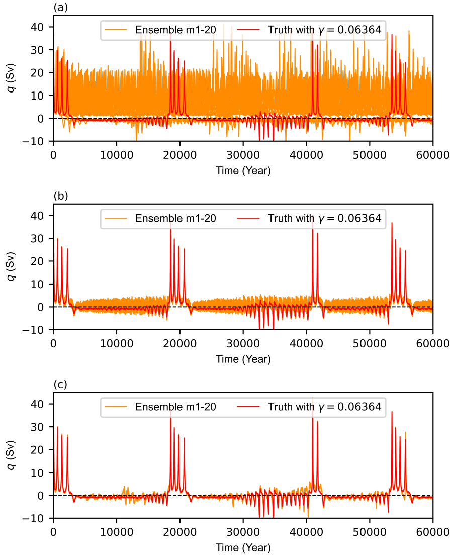
610 Figure 9. Time series of the meridional overturning circulation q in the “truth” simulation with \gamma = 0.06364 (red) and the individual ensemble 615 members (orange) in the free model control ensemble simulations a) without data assimilation and parameter estimation, b) with data assimilation or c) with data assimilation and parameter estimation using erroneously-guessed \gamma values with a Gaussian perturbation that has a mean value of 0.070004 and a standard deviation of 10% times the standard value. The dashed black line denoting q = 0 is a division line between two equilibrium states.
