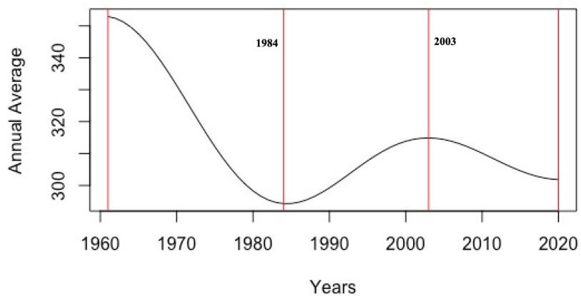
11 Figure 19: The EAWD trend as a function of the average rainfall per year
