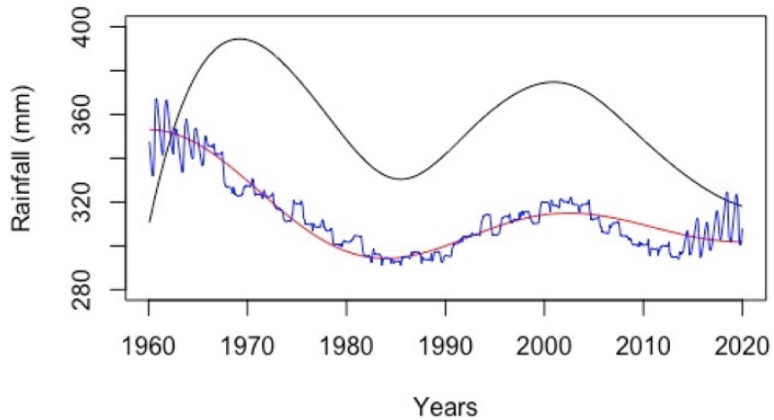
7 Figure 18: The residual Trend_{EAWD} returned by the EAWD technique (red curve), the trend of the original signal 8 obtained from a moving window (blue curve) having a size fixed at 144 (i.e. 12 years), and the residual returned by the 9 EEMD technique (black curve).
