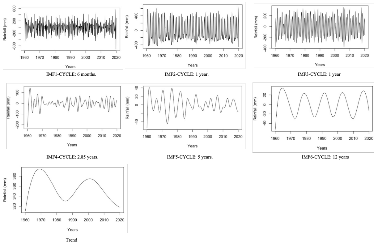
15 Figure 13: Relevant IMFs and Trend from the EEMD applied to Conakry rainfall time-series, from 1960 to 2019.
