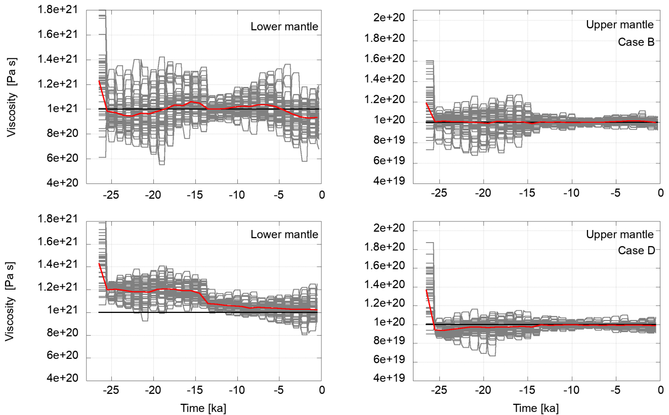
Figure 8. Development of viscosity in the lower mantle (left column) and the upper mantle (right column) for scenario two (test cases B and D, from top to bottom) in grey. The flat segments represent the viscosity values of an ensemble member during the forecast phase. When observations are available, a model state may be resampled and perturbed. This changes the viscosity values as shown. The horizontal black lines represent the viscosities of the reference experiment towards which the ensemble mean is expected to converge. The red lines are the weighted ensemble means. For the initial value all members are weighted equally. Thereafter, they are weighted by the likelihood of the observations given the current member model state.
