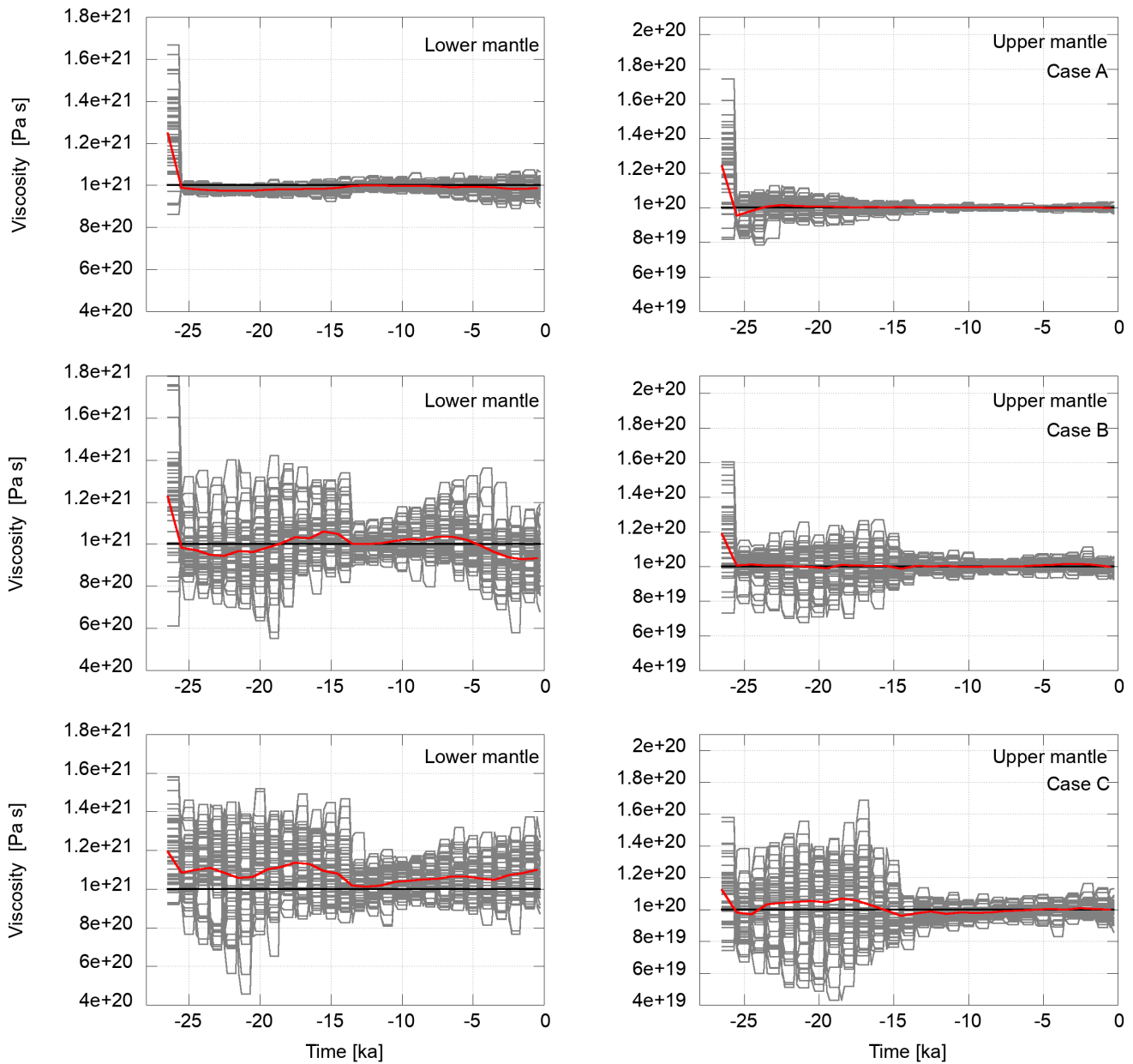
Figure 6. Development of viscosity in the lower mantle (left column) and the upper mantle (right column) for scenario one (Cases A-C, from top to bottom) in grey. The flat segments represent the viscosity values of an ensemble member during the forecast phase. When observations are available, a model state may be resampled and perturbed. This changes the viscosity values as shown. The horizontal black lines represent the viscosities of the reference experiment towards which the ensemble mean is expected to converge. The red lines are the weighted ensemble means. Ensemble members are weighted by the likelihood of the observations given the current member model state.
