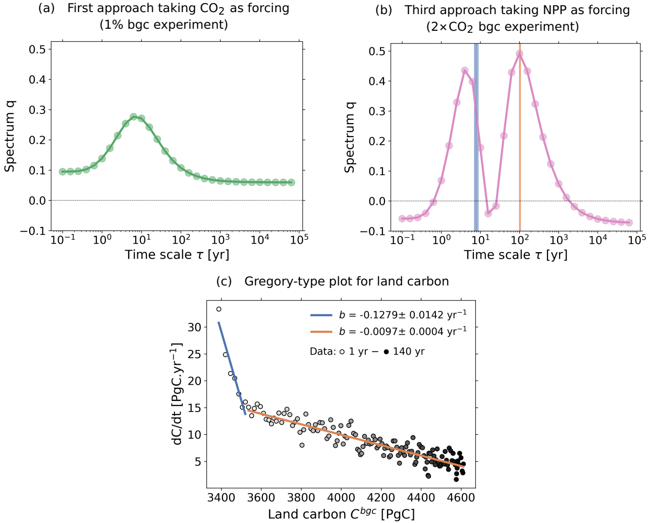
Figure 9. Spectra associated to \chi_{NPP} derived with different resolutions and a Gregory-type plot to identify the time-scale structure of land carbon. (a) Spectrum derived with the first approach (taking \text{CO}_2 as forcing) from the 1% bgc experiment; (b) Spectrum derived with the third approach (taking NPP as forcing) from the 2\times\text{CO}_2 bgc experiment; (c) Gregory-type plot of global land carbon against land-atmosphere carbon flux. Dots are the data, with the color scale from white to black indicating the evolution from 1 to 140 years. Values of b indicate the rate at which the time derivative of land carbon changes with respect to the land carbon itself. Ranges of time scales corresponding to each rate accounting for one standard deviation are shown in subfigure (b).
