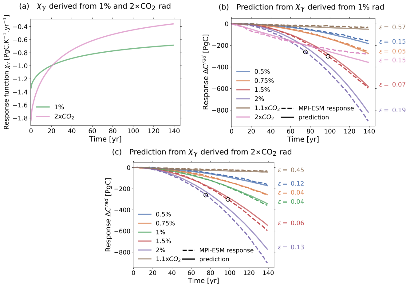
Figure 5. \chi_\gamma recovered from 1% and 2\times\text{CO}_2 rad experiments and prediction of model responses using these recoveries of \chi_\gamma . Circles indicate the maximum value for which 1.5% and 2% responses are predictable according to the estimate of the linear regime (see text). At the right of subfigures (b) and (c) the relative prediction error (see Eq. (10)) is indicated for the different experiments, calculated for the 1.5% and 2% rad experiments by considering only values preceding the circles.
