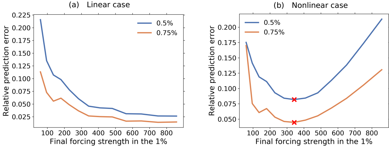
Figure 2. Toy model example for the identification of the linear regime by using additional experiments. Shown is the relative prediction error (10) for the response of 0.5% and 0.75% experiments as obtained from the response function calculated by the RFI method from 1% experiments. The relative prediction errors are plotted against the final forcing strengths of a sequence of 1% experiments with increasing time series length. The crosses at the minima indicate the final forcing strength for which the response function is optimally recovered (see text). Subfigure (a) shows the behaviour for the fully linear toy model ( a = 0 ) and subfigure (b) the behaviour in the presence of nonlinear contributions to the response ( a = 5 \times 10^{-5} ). For the purpose of demonstrating more clearly the increase in the relative prediction error for a decrease in the forcing strength, we include in the plot cases where the forcing strength is extremely small, corresponding to very small time series lengths. To deal with such cases, we set for a number of data points N < 30 the number of time scales M = N (see parameters for the RFI method in Part I). For such small number of time scales, usually no plateau in the singular values spectrum is found (step 2 of Fig. 1 in Part I). Therefore, for these special cases we also modify the algorithm to interpret the two smallest singular values as a plateau, since their small magnitude makes them have a similar effect to those singular values belonging to the plateau itself. In addition, to illustrate the most general case where \chi(t) is not known to be monotonic, we exclude here the monotonicity check (step 6 of Fig. 1 in Part I).
