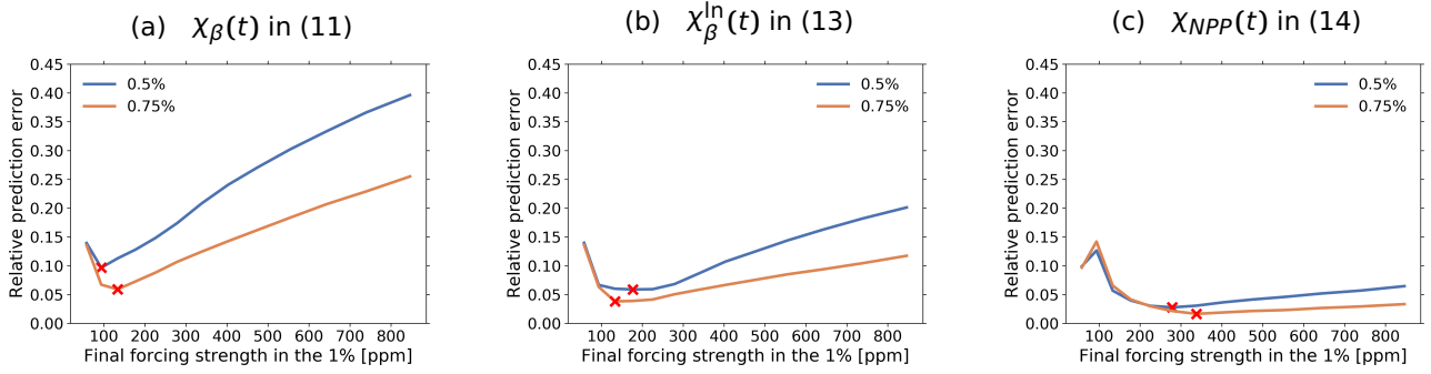
Figure 6. Prediction Relative prediction error (10) for the 0.5% and 0.75% bgc experiments obtained when using \chi_\beta(t) , \chi_\beta^{\ln}(t) and \chi_{NPP}(t) obtained from the 1% bgc experiment to predict the response. The error is shown as a function of the CO 2 final forcing strength.
