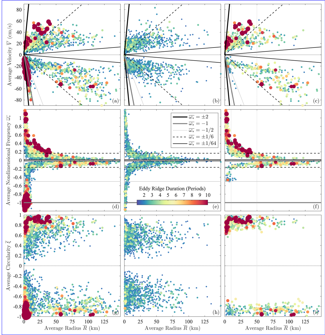
Figure 12. Scatter plots of ridge-averaged quantities from the surface drifter data (left column), together with the same plots for a noise dataset of the same size (center column), and for the surface drifter dataset after the application of the noninertial criterion \bar{\omega}_* > -1/2 together with the significance criterion \rho_X < 0.1 with X = L\bar{\xi}^4 described later in the text (right column). In (a) and (b), the location of each ridge in ridge-averaged radius \bar{R} versus ridge-averaged velocity space \bar{V} is shown, by plotting the geometric-mean radius \bar{R}_* against the kinetic-energy velocity V_* . The color and size both represent the ridge length L_*L , defined to be the number of periods an oscillation executes along the ridge. In (d) and (e), the y-axis is now the ridge-averaged nondimensional frequency \bar{\omega}_*\bar{\omega}_* , while in (g) and (h) it is the ridge-averaged circularity \bar{\xi} . Diagonal lines in the upper row, and horizontal lines in the central row, mark lines of constant \bar{\omega}_*\bar{\omega}_* , with values as given in the legend. Recall that the ridges are found for 1/64 \leq |\bar{\omega}(t)| \leq 2/64 \leq |\omega_*(t)| \leq 2 , thus the magnitudes of ridge-averaged frequencies \bar{\omega}_* must |\bar{\omega}_*| will also mostly be within that range. In the right-hand column, vertical lines at \bar{R} = 10 km and \bar{R} = 50 km denote apparent transitions between different regimes.
