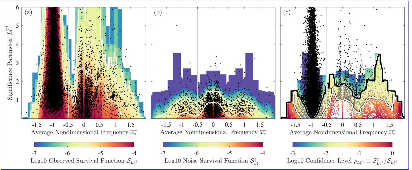
Figure 14. A significance criterion for wavelet ridges in the Gulf of Mexico surface drifter dataset. The black dots in panel (a) show the locations of all ridges in the ridge-averaged circularity-magnitude |\zeta_*| nondimensional frequency |\bar{\omega}_*| versus the product of ridge duration L_* space and fourth power of the ridge-averaged circularity , L\xi^4 . Bin-averaging to form the two-dimensional histogram in nondimensional frequency bins of width \Delta\omega = 1/4 , and then cumulatively summing this in both dimensions, but along the y-axis from high values to low values rather than the more usual low to high values , leads to an object called the complementary cumulative distribution function or survival function \mathcal{S}_*(\zeta_*, L_*) \mathcal{S}_X(x; \omega) for X = L\xi^4 , constructed here to be a function of frequency; this is shown as the colored shading in (a). White lines are the 10^{-5} and 10^{-6} contours of the survival function. Panel (b) is constructed in the same way as (a) but for the noise dataset. Since this dataset is ten times the size of the observations, for display purposes only 10% of the dots are shown, and the histogram is divided by a factor of 10, thus making these panels (a) and (b) directly comparable. Finally the logarithm of the ratio \rho_*(\zeta_*, L_*) \equiv \mathcal{S}_e / \mathcal{S}_* \rho_X(x; \omega) \equiv \hat{\mathcal{S}}_X^e(x; \omega) / \hat{\mathcal{S}}_X(x; \omega) is shown in (c). The gray-heavy white line in this panel marks the \rho(\zeta_*, L_*) = 0.1 \rho_X(x; \omega) = 0.1 contour such that only one out of ten events above or to the right of this curve is expected to be a false positive. Similarly, the black line is the \rho(\zeta_*, L_*) = 0.01 \rho_X(x; \omega) = 0.01 contour, above which only one out of 100 events is expected to be a false positive. Dots in this panel are those of the data, the same as in (a). The gray and black and gray dots mark observed ridges falling above the 0.1 and 0.01 and 0.1 contours, respectively. Those falling below the \rho(\zeta_*, L_*) = 0.1 \rho_X(x; \omega) = 0.1 contour, shown as white dots, are judged to be statistically insignificant and are rejected. The thin vertical gray line in all panels marks \omega_* = -1/2 . Events to the left of this line likely represent inertial oscillations, apparent as the prominent peak in the vicinity of \bar{\omega}_* = -1 , rather than coherent eddies.
