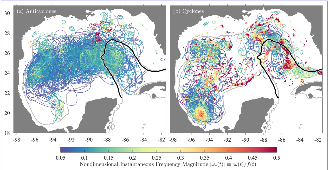
Figure 2. Ellipses from all statistically significant eddy signals in the dataset shown in Fig. 1 detected using the method described here, with anticyclonic events in (a) and cyclonic events in (b). The time interval between successive ellipses is equal to the estimated period of the oscillation, 2\pi/|\omega(t)| , where \omega(t) is the instantaneous frequency defined subsequently in Eq. (35). The colored shading is the nondimensional instantaneous frequency magnitude |\omega_*(t)| \equiv |\omega(t)/f_\circ(t)| , in which \omega(t) has been normalized by the Coriolis frequency at the latitude of the ellipse’s center, denoted f_\circ(t) . It will be shown that 2|\omega_*(t)| is an estimate of the local Rossby number of the oscillatory flow. Ellipses are plotted in reverse order of their |\omega_*(t)| value, thus placing higher-frequency, more nonlinear features on top. The asymmetry between cyclonic and anticyclonic features is strikingly apparent. Other lines are as in Fig. 1.
