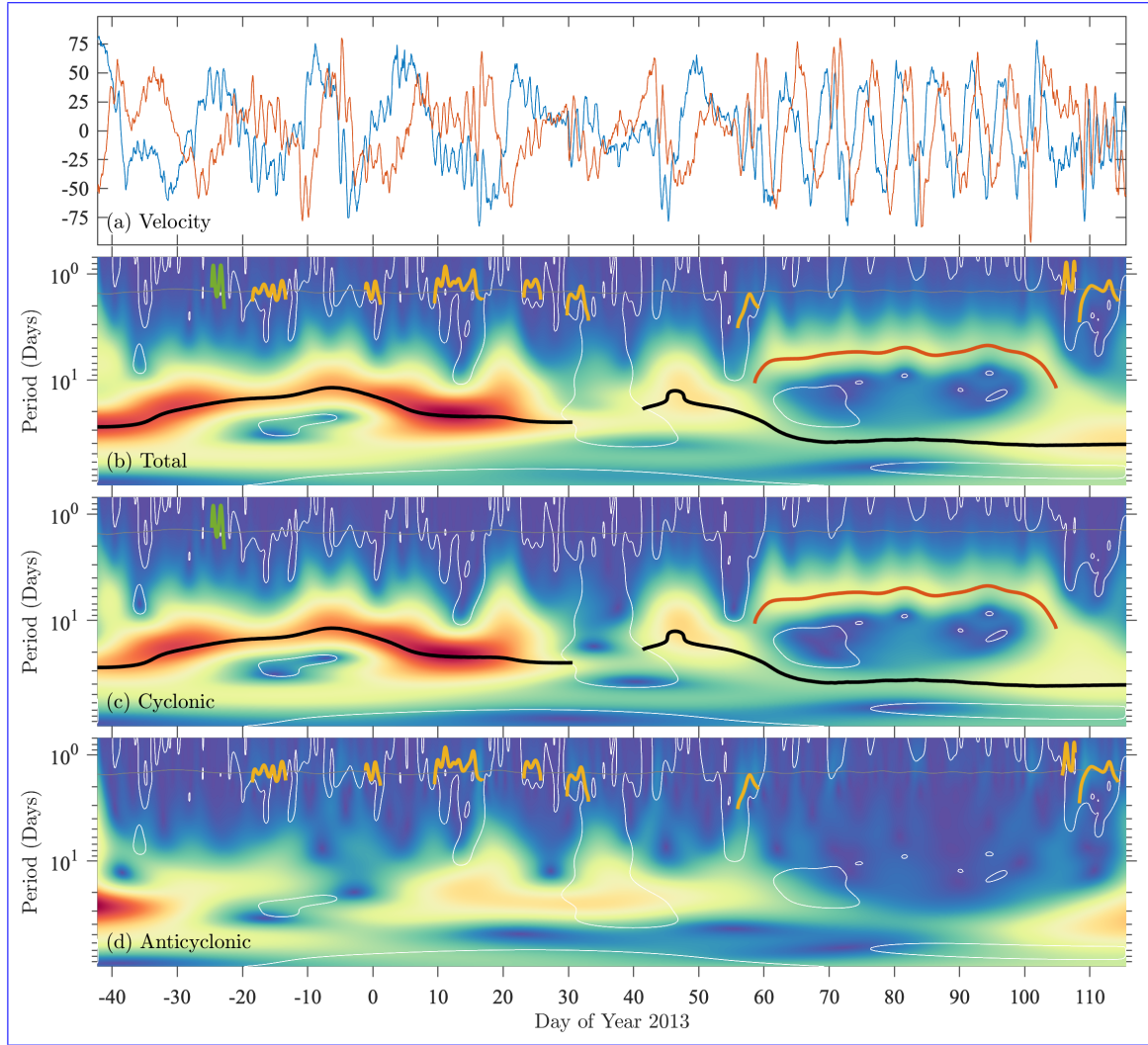
Figure 10. One-sided wavelet ridge analysis of the signal presented in Fig. 9a. In (a), the zonal and meridional velocities u(t)-v_x(t) and v(t)-v_y(t) associated with the displacement signal in Fig. 9a are shown as blue and orange curves, respectively. Panel (b) shows the total wavelet transform magnitude, \|\mathbf{w}(t, s)\| = \sqrt{|w^+(t, s)|^2 + |w^-(t, s)|^2} , while (c) and (d) show the magnitudes of the positive (or cyclonic) and negative (or anticyclonic) rotary transforms, |w^+(t, s)| and |w^-(t, s)| . The y-axis in all of these plots panels (b)–(d) is scale converted to oscillation period, 2\pi s/\omega_{\beta, \gamma} . The thin, nearly horizontal gray line in panels (b)–(d) marks the scale location of the time-varying Coriolis frequency f(t) period 2\pi/f(t) , while the thin white lines mark the curves where the magnitudes of the two rotary transforms are equal, |w^+(t, s)| = |w^-(t, s)| . The colored lines show all detected ridges \hat{s}(t) of \|\mathbf{w}(t, s)\| using the same color scheme as in Fig. 9b. There are two sets of ridges, those detected in \|\mathbf{w}(t, s)\| when the positive rotary transform w^+(t, s) dominates, and those detected in \|\mathbf{w}(t, s)\| when the negative rotary transform w^-(t, s) dominates. To show their different origins, the ridges are superposed on the dominant transform as well as being drawn on the total transform \|\mathbf{w}(t, s)\| . A condition of the one-sided algorithm is that the ridges terminate when they encounter the thin white lines, prohibiting transitions in rotation sense.
