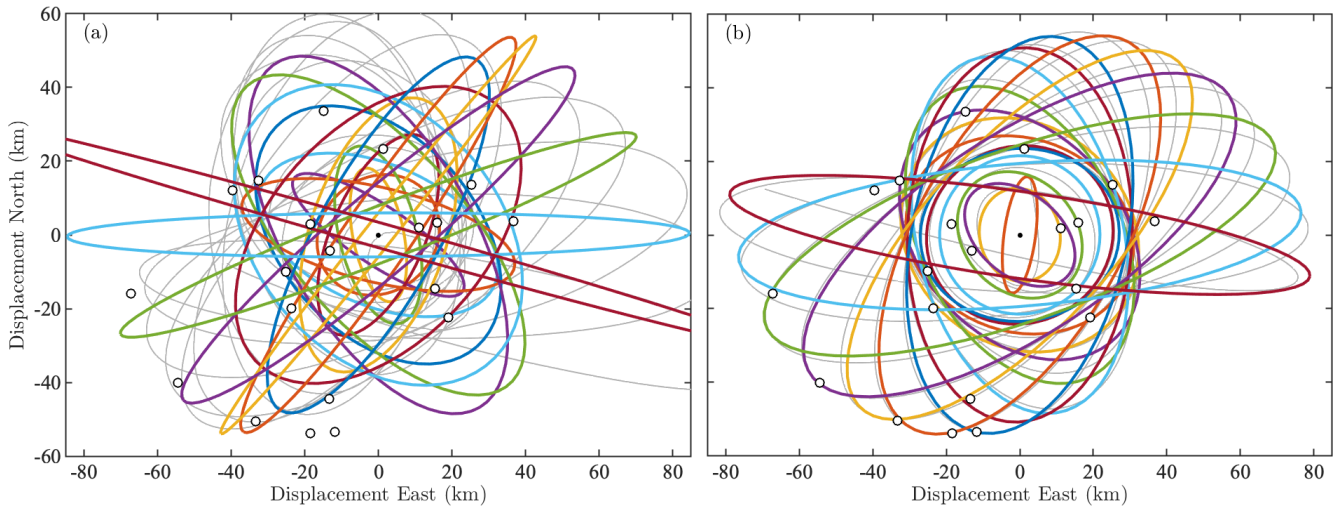
Figure 6. Ellipses inferred from the composite signal in Fig. 5a using (a) the analytic signal method directly or (b) the wavelet ridge method formulated in of Sect. 3. The gray line in each panel is the estimated modulated elliptical signal using that method, while the two respective methods. The dots are as in Fig. 4b.
