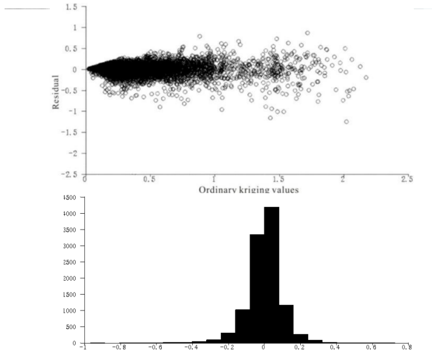
The cross-validation results: (a) residual VS Cu grade;(b) the residual distribution histogram.
