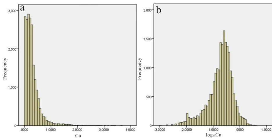
The histogram of the Cu raw (a) and logarithmic transformation (b) data.
