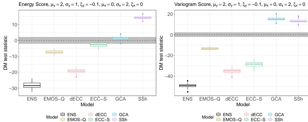
Figure 7. As Figure 6, but based on ES and VS for (\mu_y, \xi_y, \sigma_y) = (2.0, -0.1, 1.0) and (\mu_x, \xi_x, \sigma_x) = (0.0, 0.0, 2.0) , where \rho_y = 0.75 and \rho_x = 0.25
