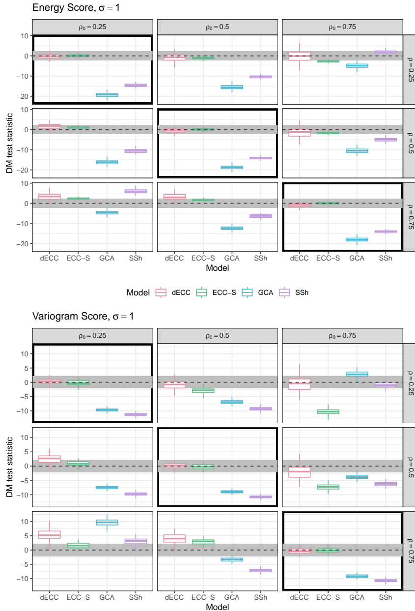
Figure 8. Summaries of DM test statistic values based on the ES (top) and the VS (bottom) for Setting 4 with \epsilon = 1 and \sigma = 1 . ECC-Q forecasts are used as reference model such that positive values of the test statistic indicate improvements over ECC-Q and negative value indicated deterioration of forecast skill. Boxplots summarize results of the 100 Monte Carlo repetitions of each individual experiment. The horizontal gray stripe indicates the acceptance region of the two-sided DM test under the null hypothesis of equal predictive performance at a level of 0.05. Simulation parameter choices where the correlation structure of the raw ensemble is correctly specified ( \rho = \rho_0 ) are surrounded by black boxes.
