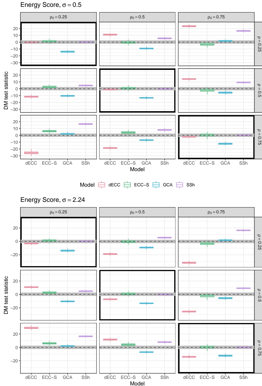
Figure 3. Summaries of DM test statistic values based on the ES for Setting 1 with \epsilon = 1 , and \sigma = 0.5 (top), and \sigma = \sqrt{5} (bottom). ECC-Q forecasts are used as reference model such that positive values of the test statistic indicate improvements over ECC-Q and negative value indicated deterioration of forecast skill. Boxplots summarize results of the 100 Monte Carlo repetitions of each individual experiment. The horizontal gray stripe indicates the acceptance region of the two-sided DM test under the null hypothesis of equal predictive performance at a level of 0.05. Simulation parameter choices where the correlation structure of the raw ensemble is correctly specified ( \rho = \rho_0 ) are surrounded by black boxes.
