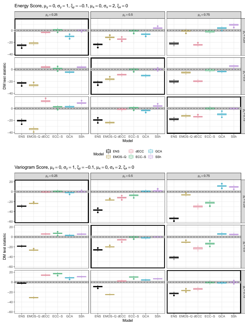
Figure 6. Summaries of DM test statistic values based on the ES (top) and the VS (bottom) for setting B from Table 1. ECC-Q forecasts are used as reference model such that positive values of the test statistic indicate improvements over ECC-Q and negative value indicated deterioration of forecast skill. Boxplots summarize results of the 100 Monte Carlo repetitions of each individual experiment. The horizontal gray stripe indicates the acceptance region of the two-sided DM test under the null hypothesis of equal predictive performance at a level of 0.05.
