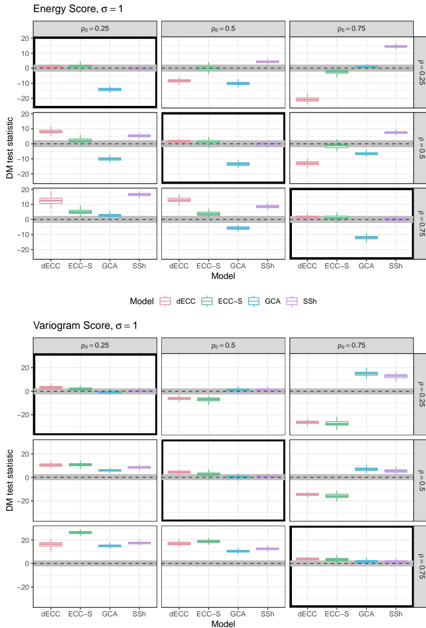
Figure 5. Summaries of DM test statistic values based on the ES (top) and the VS (bottom) for Setting 2 with \epsilon = 3 , \mu_0 = 2 , and \sigma = 1 . ECC-Q forecasts are used as reference model such that positive values of the test statistic indicate improvements over ECC-Q and negative value indicated deterioration of forecast skill. Boxplots summarize results of the 100 Monte Carlo repetitions of each individual experiment. The horizontal gray stripe indicates the acceptance region of the two-sided DM test under the null hypothesis of equal predictive performance at a level of 0.05. Simulation parameter choices where the correlation structure of the raw ensemble is correctly specified ( \rho = \rho_0 ) are surrounded by black boxes.
