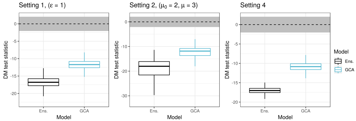
Figure 1. Summaries of DM test statistic values based on the CRPS. ECC-Q forecasts are used as reference model such that positive values of the test statistic indicate improvements over ECC-Q and negative value indicated deterioration of forecast skill. Boxplots summarize results of from multiple parameter combinations for the simulation settings, with restrictions on the simulation parameters indicated in the plot title. For example, boxplots in the first panel summarize simulation results from all parameter combinations of Setting 1 (and the 100 Monte Carlo repetitions each) subject to \epsilon = 1 . The horizontal gray stripe indicates the acceptance region of the two-sided DM test under the null hypothesis of equal predictive performance at a level of 0.05.
