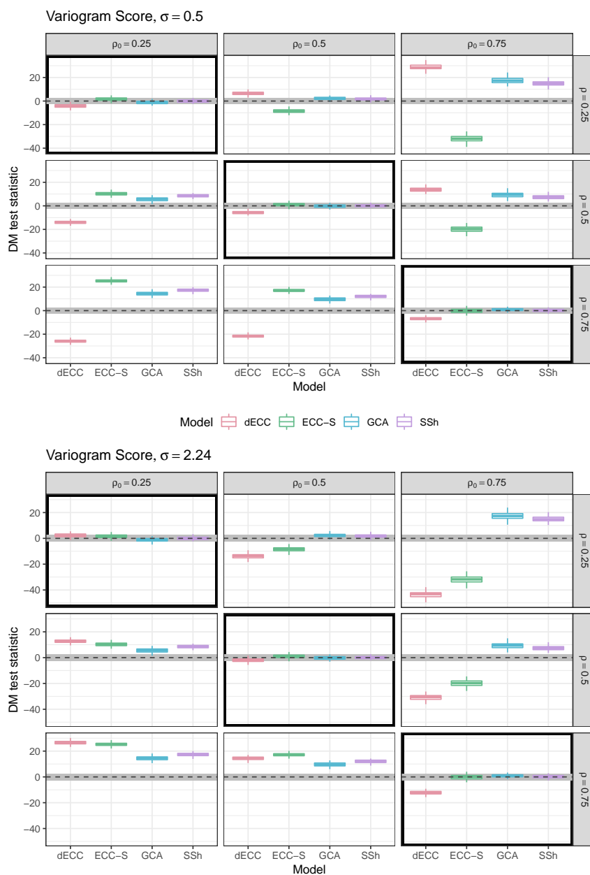
Figure 4. As Figure 3, but summarizing results in terms of the VS.
