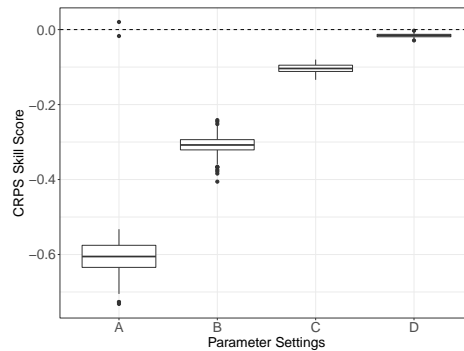
Figure 2. CRPS skill score of raw ensemble with ECC-Q as reference model for the four different scenarios considered in Setting 3. The boxplots summarize results over 100 repetitions of each individual experiment.
