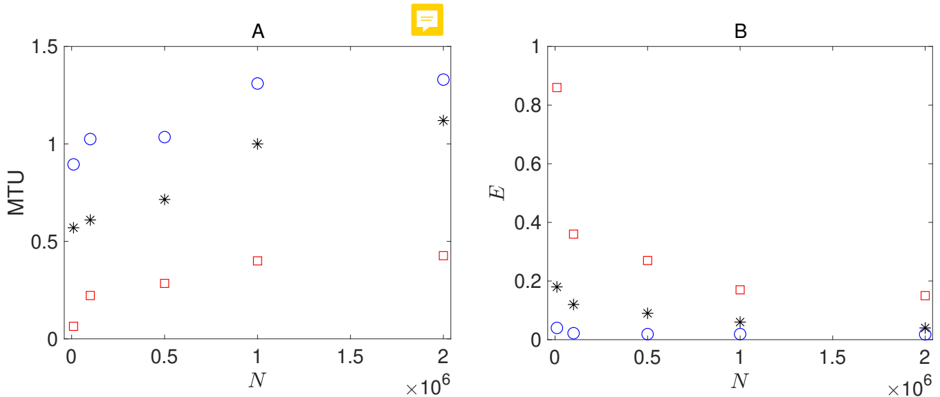
Figure 7. Comparison of the short-term prediction quality for RC-ESN (blue circles), RNN-LSTM (black stars), and ANN (red squares) as the size of the training set N is changed from N = 10^4 to N = 2 \times 10^6 . (A) Prediction horizon (when e(t) reaches 0.3). (B) Average error E (see Eq. (10)). The hyperparameters in each method are optimized for each N .
