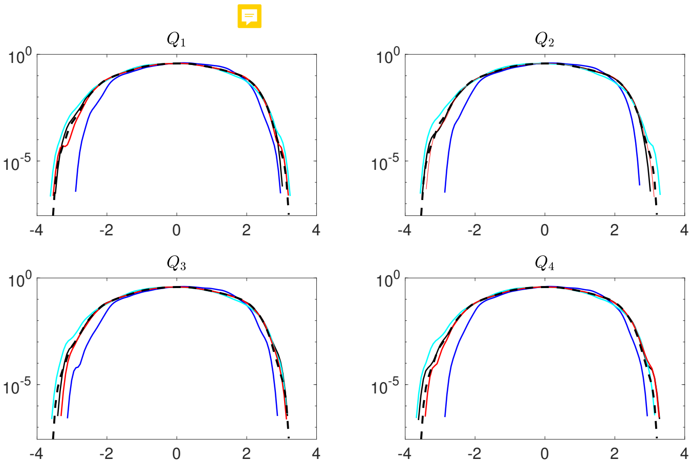
Figure 9. Estimated probability density functions (PDFs) of long datasets freely predicted using RC-ESN (red), ANN (blue), and RNN-LSTM (cyan) compared to the true PDF (dashed black). RC-ESN, ANN, and RNN-LSTM are first trained with N = 500000 , and then predict, from an initial condition, for 4 \times 10^6 \Delta t . The panels Q_1 - Q_4 correspond to the equally divided quartiles of 10^6 predicted samples. PDFs are approximated using kernel density estimation (Epanechnikov, 1969). The green lines show the estimated PDFs from different sets of 10^6 samples that are obtained from numerical solution of Eqs. (1)-(3). Small differences between the green lines show the uncertainties in estimating the tails from 10^6 samples. The dashed black lines show the true PDF estimated from 10^7 samples from numerical solution. Note that the presented PDFs are for standardized data.
