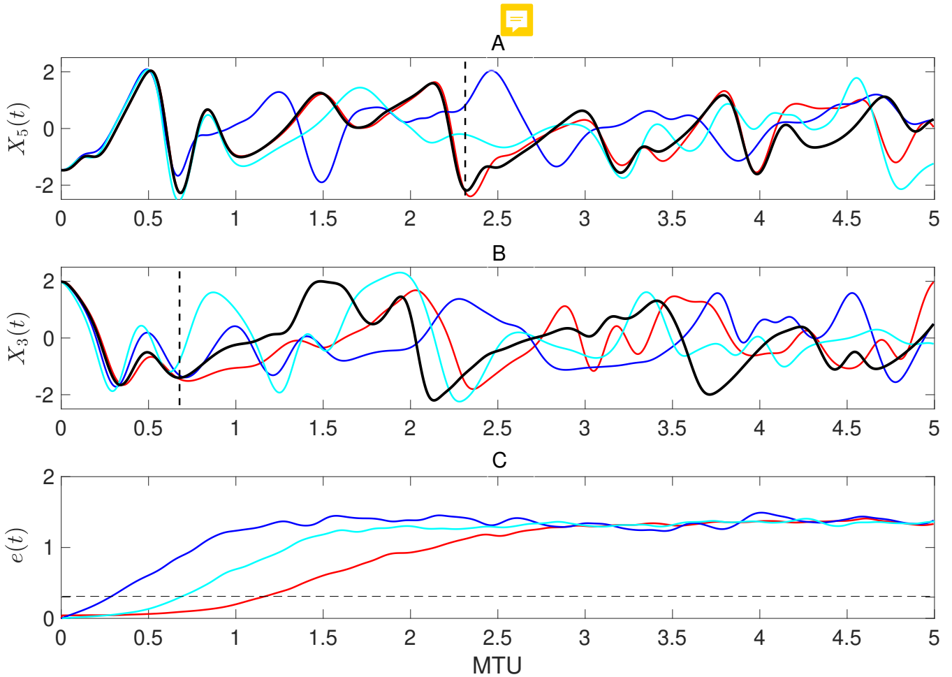
Figure 5. Comparison of the short-term forecast skills among the three deep learning methods. The lines show truth (black), RC-ESN (red), ANN (blue), and RNN-LSTM (cyan). (A) and (B) show examples (differing in initial condition) for which RC-ESN yields the longest and shortest prediction horizons, respectively. Vertical dashed lines approximately show the prediction horizon of RC-ESN. (C) Relative L_2 error averaged over 100 randomly chosen initial conditions e(t) (see Eq. (9)). The dashed horizontal line marks e = 0.3 . Time is in MTU, where 1 \text{ MTU} = 200\Delta t \approx 4.5/\lambda_{max} . Training size is N = 500000 .
