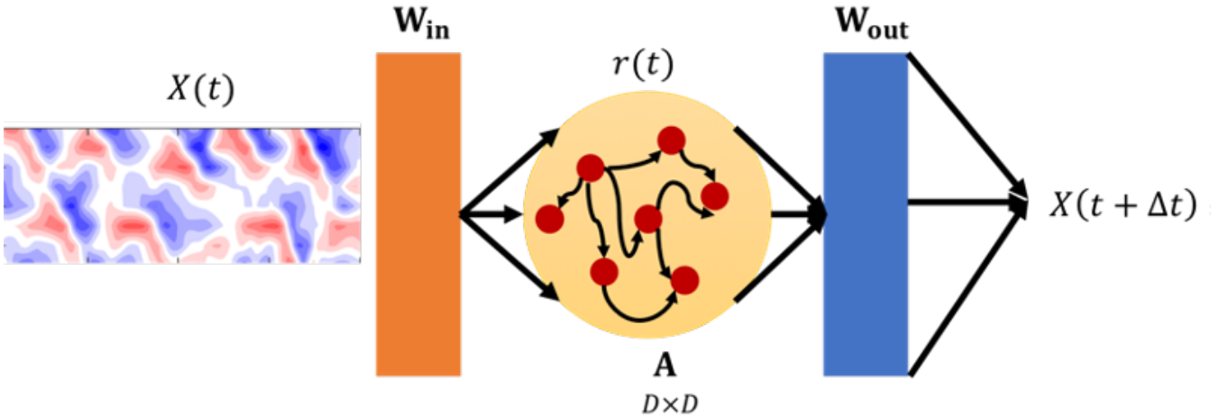
Figure 3. A schematic of RC-ESN. D \times D is the size of the adjacency matrix of the reservoir \mathbf{A} . X(t) ( -T \leq t \leq 0 ) is the input during training. \mathbf{W}_{\text{in}} and \mathbf{A} are random matrices that are chosen at the beginning of training and fixed during training and testing. Only \mathbf{W}_{\text{out}} is computed during training. During testing ( t > 0 ), X(t + \Delta t) is predicted from a given X(t) that is either known from the initial condition or has been previously predicted.
