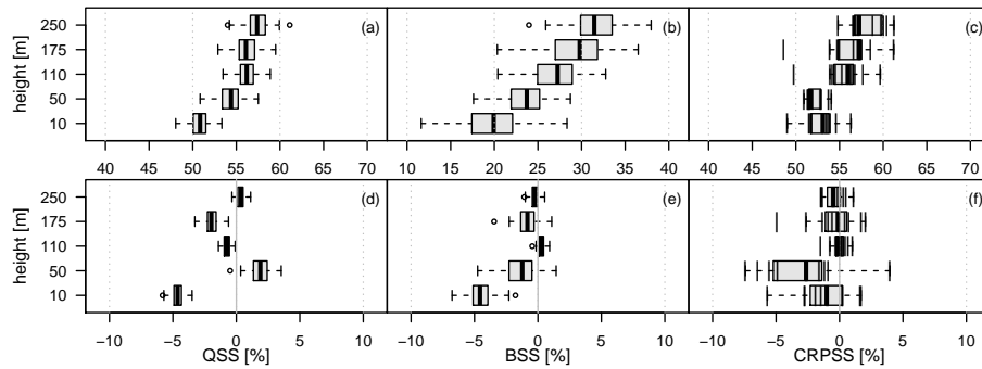
Figure 5. Verification skill scores for Legendre model against climatology (a) to (c) and against layer-wise model (d) to (f). The QSS is given for the predictive \tau = 99\% -quantile in (a) and (d); the BSS for thresholds corresponding to the observations 99%-quantile ( u = 14.8 m/s in 10 m, u = 19.26 m/s in 50 m, u = 21.01 m/s in 110 m, u = 22.55 m/s in 175 m, u = 23.97 m/s in 250 m) in (b) and (e); and the CRPSS in (c) and (f). For QSS and BSS the box-whiskers represent the 100 member bootstrap sample, with the box giving the inner quartile range. The range of the whiskers is maximal 1.5-times the width of the box. For the CRPSS the boxes represent the eleven cross-validated estimates.
