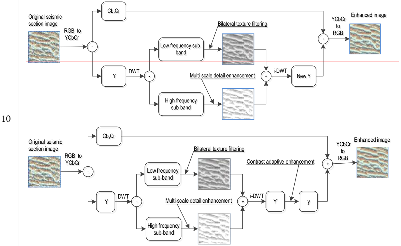
Fig. 1 Process of seismic section image detail enhancement
