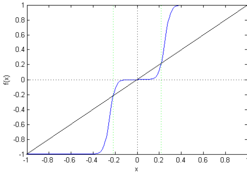
Fig. 3 The graph of adaptive enhancement transform function, in which b = 0.25 , c = 40
