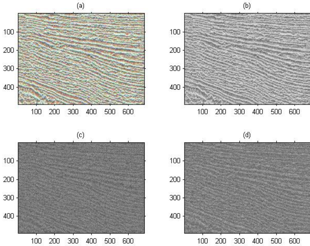
5 Fig. 4 Converting a seismic section image from RGB format to YcbCr format; (a) Original seismic image; (b) The brightness component Y of the image (a) after the format conversion; (c), (d) Chroma component Cb and Cr of image (a) after format conversion
