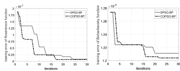
Fig. 1 Training error curves of SPSO-BP and COPSO-BP algorithms
