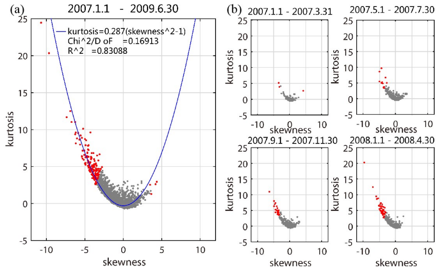
Figure 6. Negentropy distributions in the skewness-kurtosis domain in (a) January 1, 2007, to June 30, 2009, and (b) four shorter periods before the earthquake. Red denotes that the negentropy is greater than k^* , and grey indicates that the negentropy is less than k^* . The blue curve is the quadratic fit with a 95% confidence.
