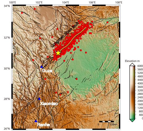
Figure 1. Location map showing the epicentre of the Wenchuan earthquake epicentre and the Guza station three stations. The Wenchuan earthquake occurred at 14:28:04 on May 12, 2008 (UTC+8). The magnitude of the earthquake was Ms 8.0, and the focal depth was approximately 14 km. The epicentre was located in Wenchuan County, Sichuan Province, at 31.01°N, 103.42°E shown by yellow star. The blue rectangles show the strainmeter stations. The red circles are aftershock distribution from the main shock on May 12, to October 30, 2008. The green curve is the schematic curve of the main rupture zone and black curves are faults.
