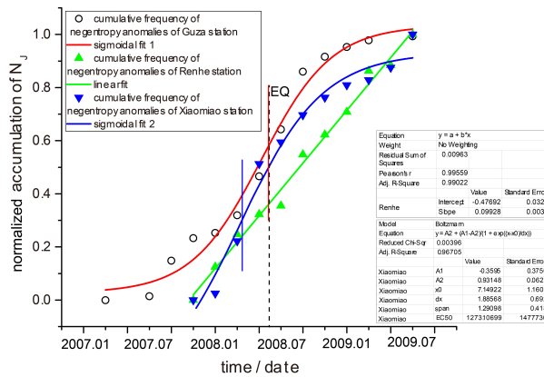
Figure 10. Cumulative frequency of negentropy anomalies of Xiaomiao station and Renhe station from September 16, 2007 to June 30, 2009. The negentropy analysis of Guza station is from January 1, 2007 to June 30, 2009, because of the different installation time of the instruments. The red vertical line is the inflection point of the fitting curve of Guza station. The blue vertical line is the inflection point of the fitting curve of Xiaomiao station. The black dotted line is the earthquake day.
