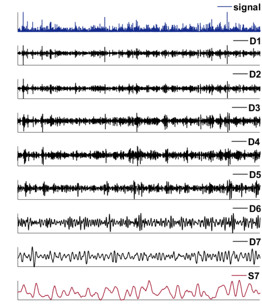
10 Figure 2 Scheme of multi-scale decomposition of signals using maximum overlap discrete wavelet transformation (MODWT). The relationship between signal Y_t (blue), detailed component D_j (black), and approximate component S_j (red), is shown.
