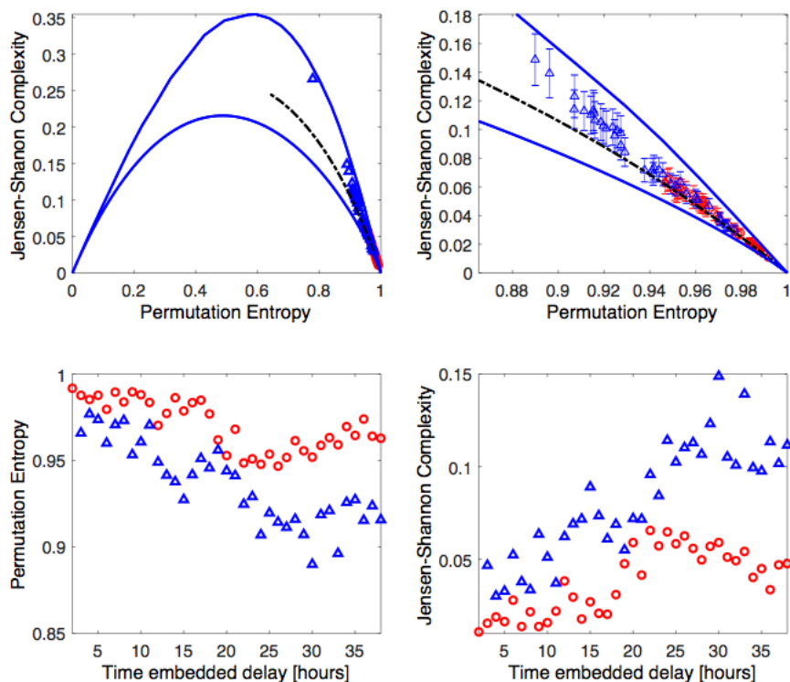
Figure 5. Jensen-Shannon complexity and permutation entropy for S_{(1)} (black square), AL (red) and am (blue) for 500 points with no gaps sampled at 1 hour interval, embedding dimension d=4 and embedding delays ranging between 2 hours and 40 hours.
