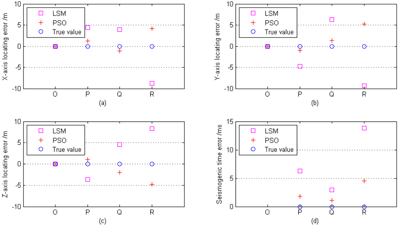
5 Fig. 3 Comparisons of the errors in the source location parameters between the LSM and PSO algorithms: (a) Comparisons of the x-axis locating error; (b) Comparisons of the y-axis locating error; (c) Comparisons of the z-axis locating error; (d) Comparisons of the errors in the origin time estimation.
