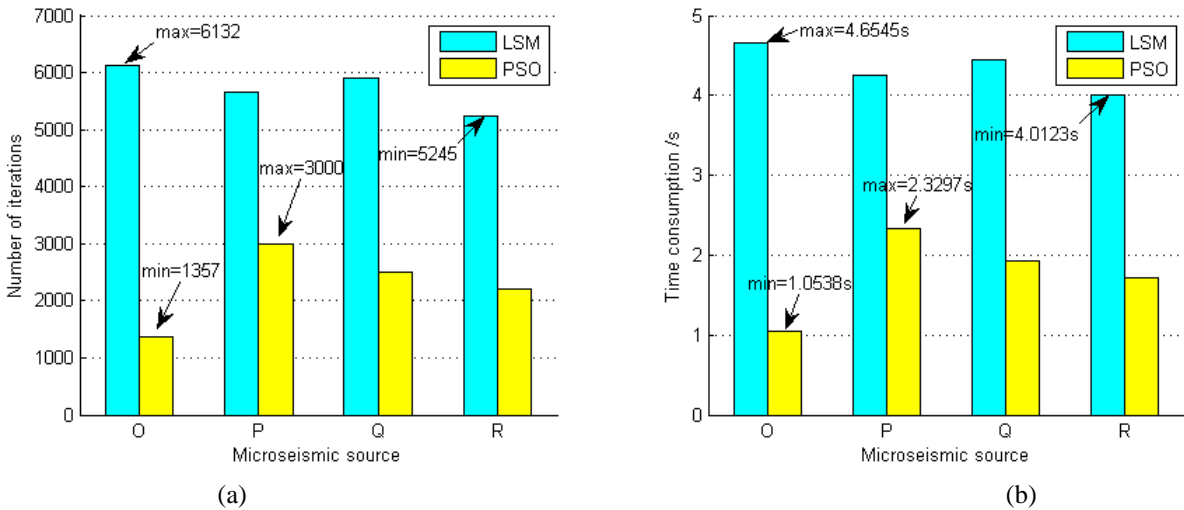
10 Fig. 4 (a) Comparison of the number of iterations between the LSM and PSO algorithms, where the max and min markers are highlighting the max and min number of iterations for each algorithm; (b) Comparison of the computing time between the LSM and PSO algorithms, where the max and min markers are highlighting the max and min amount of computing time for each algorithm.
