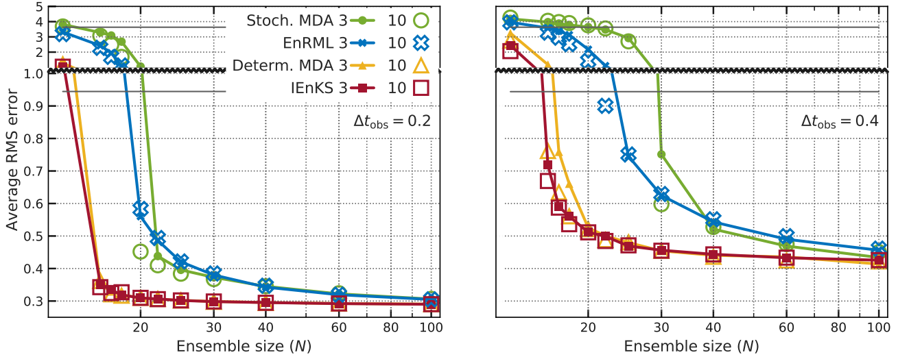
Figure 1. Benchmarks of the (filtering) accuracy of four iterative ensemble smoothers, obtained with the Lorenz-96 system, plotted as functions of N . The y -axis changes resolution at y = 1 . For perspective, the two lines at y = 3.6 and y = 0.94 show the average RMSE of the climatological mean, and of the optimal interpolation method, respectively. Each of the iterative ensemble smoothers is plotted for 3 (compact markers) and 10 (hollow markers) iterations. It can be seen that the deterministic (i.e. square-root) methods systematically achieve lower RMSE averages.
