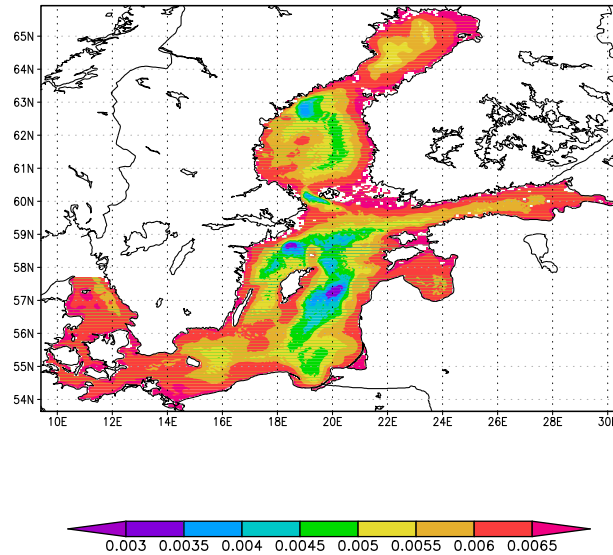
Figure 1. The gradient of the functional G(T) [ \text{m}^{-2}\text{s}^{-1} ]
