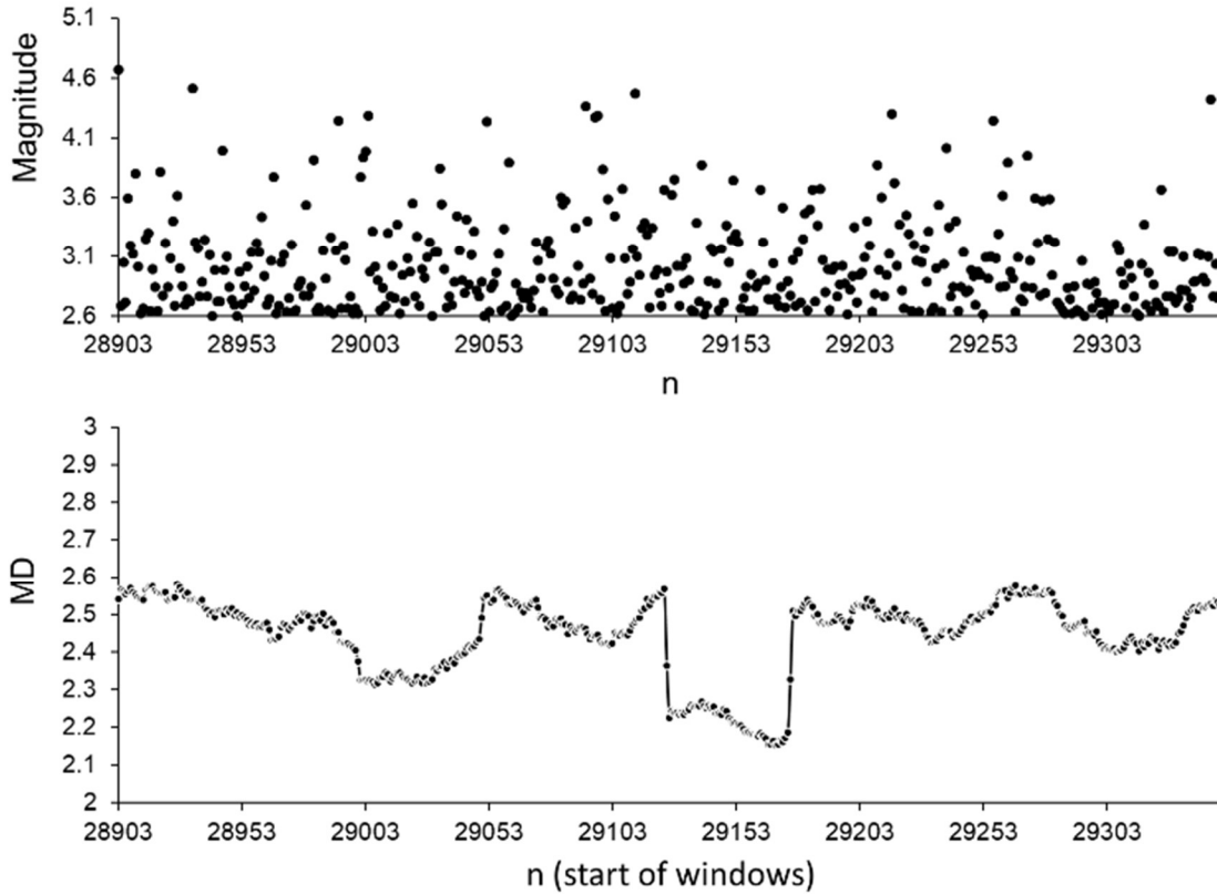
395 Fig. 12. Magnitudes and MD values calculated for part of the SC catalogue after M7.2 (04.04.2010, sequential number in SC catalogue 28129) from 06.04.2010 (sequential number in SC catalogue 28903) to 08.04.2010 (sequential number in SC catalogue 29350). Average MD values were calculated for 50 data windows, shifted by one data step. 99% of the earthquakes in this period occurred within a distance of 0.7–60 km from the epicentre of M7.2.
