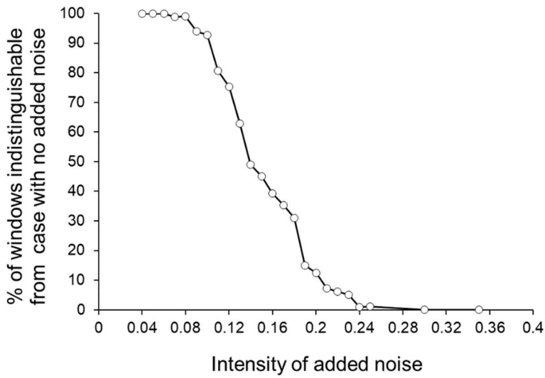
235 Fig. 4. The percentage of the 50 data windows (shifted by 50 data steps) of the crack fusion model with added noise that are indistinguishable from the initial condition (system with no added noise).
