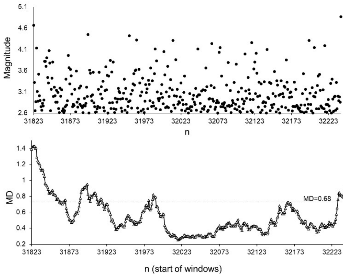
Fig. 14. Magnitudes and MD values calculated for the non-aftershock part of the SC catalogue from 07.04.2011 (sequential number in SC catalogue 31823) to 14.02.2012 (sequential number in SC catalogue 32240). Average MD values are calculated for 50 data windows, shifted by one data step.
