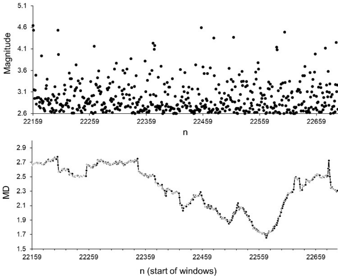
385 Fig. 11. Magnitudes and MD values calculated for part of the SC catalogue after M7.1 (16.10.1999, sequential number in the SC catalogue 21937) from 16.10.1999 (sequential number in the SC catalogue 22159) to 21.10.1999 (sequential number in the SC catalogue 22697). Average MD values are calculated for 50 data windows, shifted by one data step. 92% of earthquakes in this period occurred within a distance of 1.2–60 km from the epicentre of M7.1
