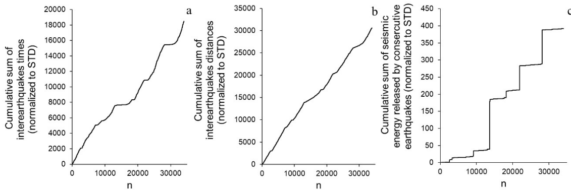
Fig. 2. Cumulative sums of (a) interevent times; (b) inter-earthquake distances; and (c) released seismic energies, starting from the first event in the southern California catalogue (1975-2017).
