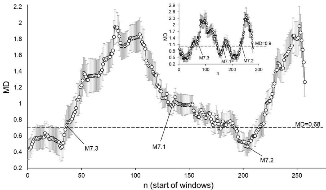
465 Fig. 17. Average MD values calculated by comparing ICT(i) , ICD(i) and ICE(i) sequences from the original SC catalogue and from the set of randomised catalogues (completeness threshold M4.6). The dotted line corresponds to a significant difference between windows at p=0.01 . MD values are calculated for 50 data windows shifted by one data step. The inset shows results calculated for 30 data windows shifted by one data step.
