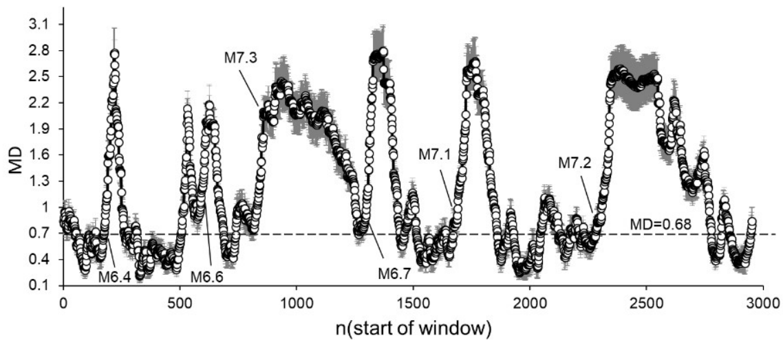
Fig. 16. Average MD values calculated by comparing ICT(i) , ICD(i) and ICE(i) sequences from the original SC catalogue and from the set of randomised catalogues (completeness threshold M3.6). The dotted line corresponds to a significant difference between windows at p=0.01 . MD values are calculated for 50 data windows shifted by one data step.
