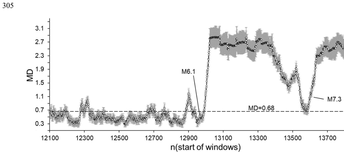
Fig. 7. Average MD values calculated for the period from 14.05.1990 (12100) to 28.06.1992 (13797) in which two strong earthquakes occurred: M6.1 (23.04.1992) and M7.3 (28.06.1992). MD values are calculated by comparing ICT(i) , ICD(i) and ICE(i) sequences from the original SC catalogue and from the set of randomised catalogues. The dotted line corresponds to a significant difference between windows at p=0.01 . MD values are calculated for 50 data windows shifted by one data step.
