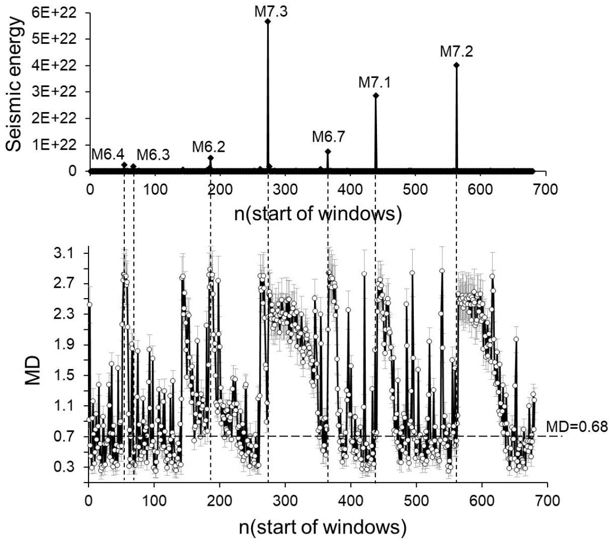
260 Fig. 5. Seismic energy released (upper curve) and average MD values (bottom curve) calculated for consecutive non-overlapping 50 data windows, shifted by 50 data steps, for the southern California earthquake catalogue (1975–2017). Averages of the MD values and the corresponding standard deviations (given in the lower plot by white circles and grey error bars) were calculated by comparing ICT(i), ICD(i) and ICE(i) sequences in the original catalogue and in the set of randomised catalogues. The dotted line corresponds to a significant difference between windows at p=0.01 .
