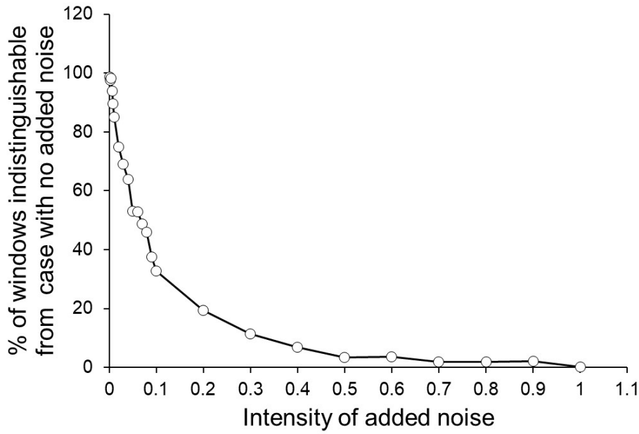
230 Fig. 3. Percentage of the 50 data windows (shifted by 50 data steps) of the Lorenz system with added noise that are indistinguishable from the initial condition (system with no added noise).
