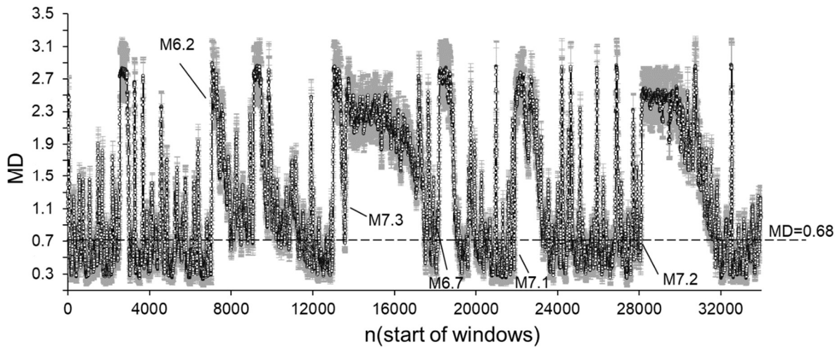
Fig. 6. Average MD values calculated by comparing ICT(i) , ICD(i) and ICE(i) sequences from the original SC catalogue and from the set of randomised catalogues. The dotted line corresponds to a significant difference between windows at p=0.01 . MD values are calculated for 50 data windows shifted by one data step.
