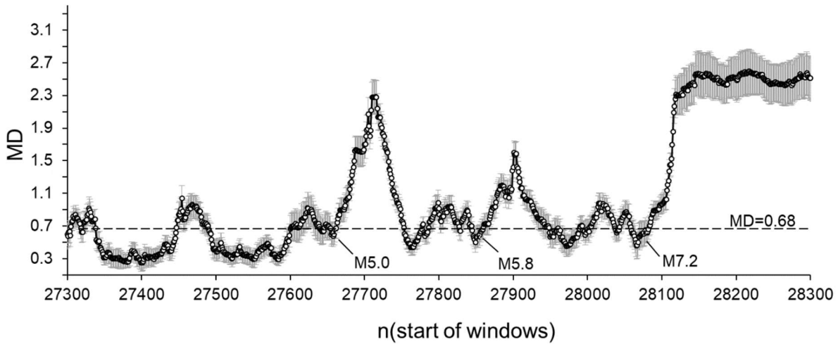
350 Fig. 9. Average MD values calculated for the period from 30.10.2008 (27300) to 05.04.2010 (28300) in which three moderate and strong earthquakes occurred: M5.0 (01.10.2009), M5.8 (30.12.2009) and M7.2 (04.04.2010). MDs are calculated by comparing ICT(i) , ICD(i) and ICE(i) sequences from the original SC catalogue and from the set of randomised catalogues. The dotted line corresponds to a significant difference between windows at p=0.01 . MD values are calculated for 50 data windows shifted by one data step.
