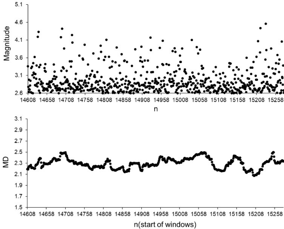
Fig. 10. Magnitudes and MD values calculated for part of the SC catalogue after M7.3 (28.06.1992, sequential number in the SC catalogue 13648) from 01.07.1992 (sequential number in the SC catalogue 14608) to 05.07.92 (sequential number in the SC catalogue 15280). Average MD values are calculated for 50 data windows, shifted by one data step. 90% of the earthquakes in this period occurred within a distance of 0.5–70 km from the epicentre of M7.3.
