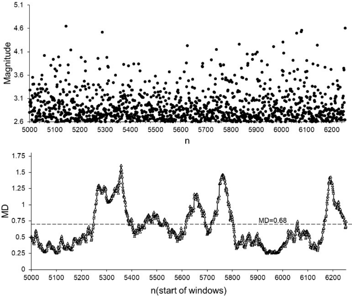
415 Fig. 13. Magnitudes and MD values calculated for the non-aftershock part of the SC catalogue from 07.03.1983 (sequential number in SC catalogue 5000) to 05.02.1985 (sequential number in SC catalogue 6253). Average MD values are calculated for 50 data windows, shifted by one data step.
