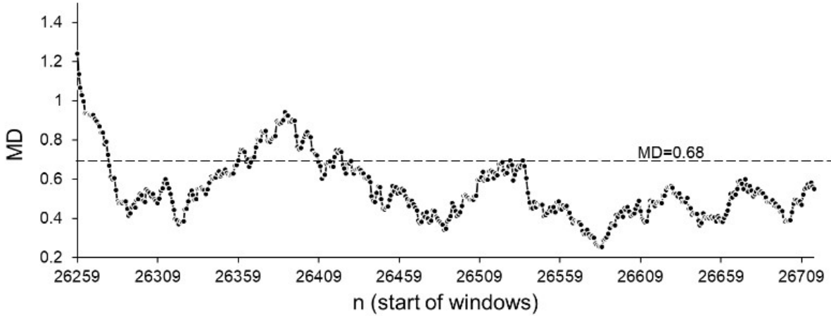
Fig. 15. Magnitudes and MD values calculated for the non-aftershock part of the SC catalogue from 24.05.2006 (sequential number in SC catalogue 26259) to 05.08.2007 (sequential number in SC catalogue 26717). Average MD values are calculated for 50 data windows, shifted by one data step.
