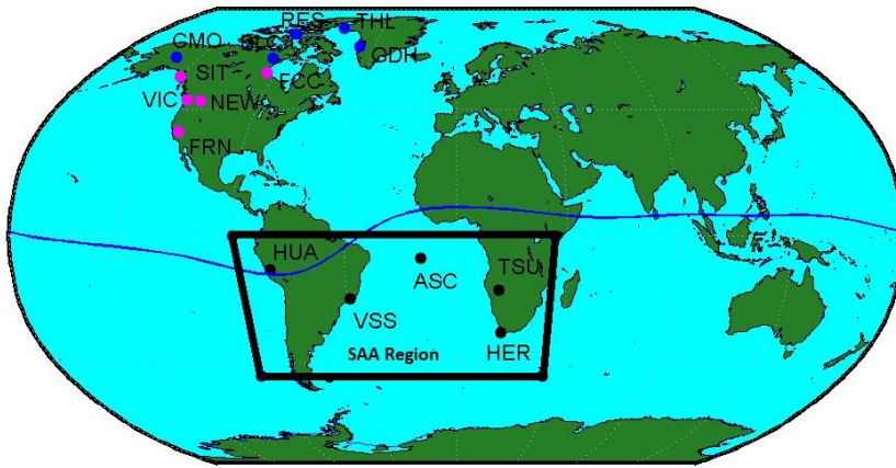
Figure 1: SAA is situated at an altitude of 200-800 km over the earth's surface. It extends as of 0 to -50 degrees of latitude along with -90 to 40 degrees of longitude. The black circle is the station in the SAA region.
