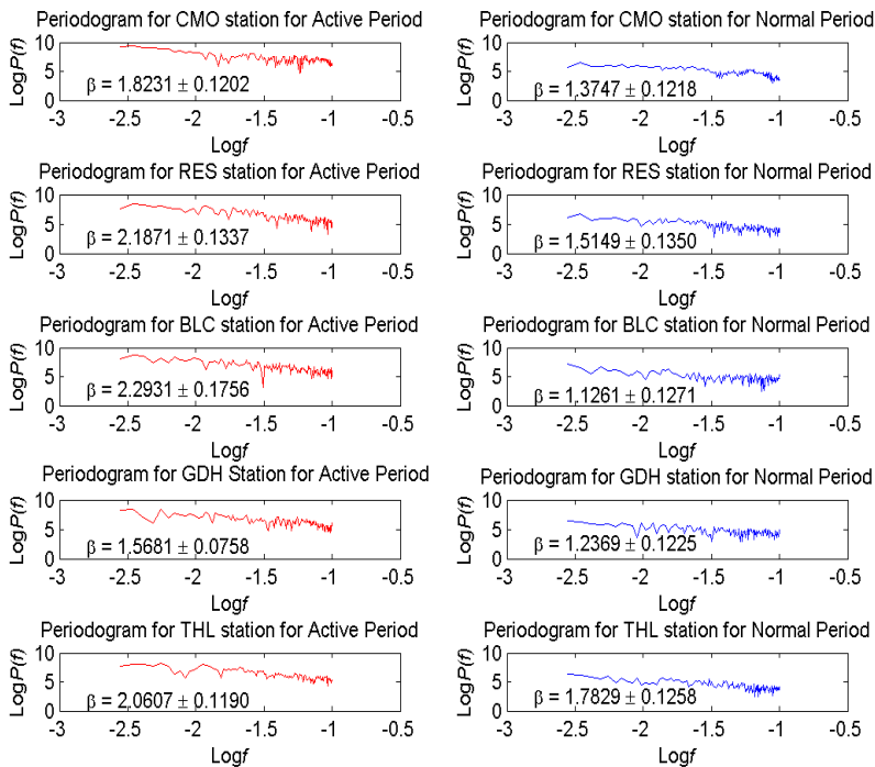
Figure 6: Periodogram for high region during active period and normal period.
