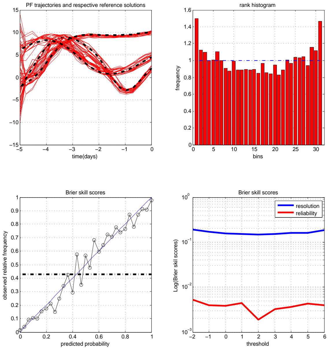
Fig. 11: Same as Figure 9, for the Particle Filter.
