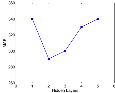
Figure 7. SFSDSA hidden layer number and MAE values.
