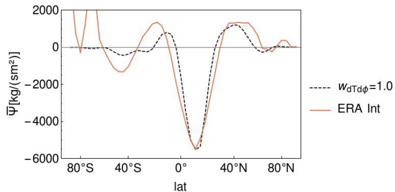
Fig. 2 Integrated northward mass flux in lower troposphere. Black: Model output for w_{T\phi} = 1 and w_{azonal} = 1 . Red: ERA Interim climatological winter data.
