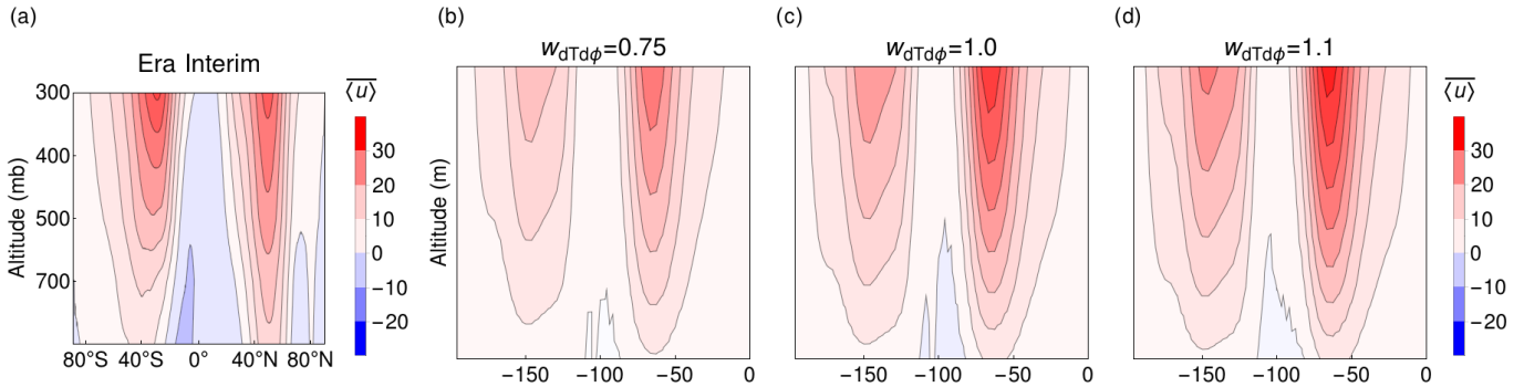
Fig. 5 Zonal mean zonal wind velocity \langle \bar{u} \rangle representing the jet streams. The subpanel (a) shows ERA-Interim data, the others results from Aeolus with different w_{T\phi} . In (b) w_{T\phi} = 0.75 , in (c) w_{T\phi} = 1.0 and in (d) w_{T\phi} = 1.1 . All other parameters are set to standard values.
