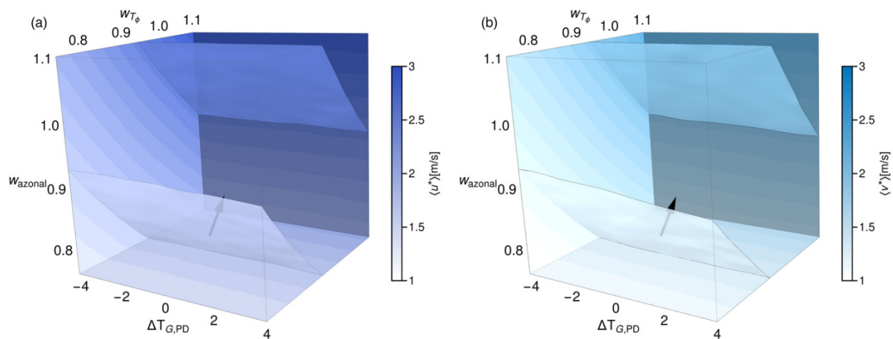
Fig. 9 Strength of planetary waves \langle u^* \rangle and \langle v^* \rangle in dependence of w_{T\phi} and w_{azonal} and \Delta T_{G,PD} . The arrow points in the direction of the strongest gradient.
