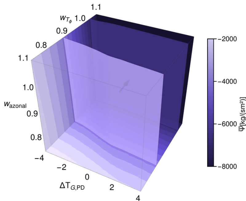
5 Fig. 4 Strength of the Hadley cell in dependence of w_{T_\phi} and w_{azonal} and \Delta T_{G,PD} . The arrow points in the direction of the strongest gradient.
