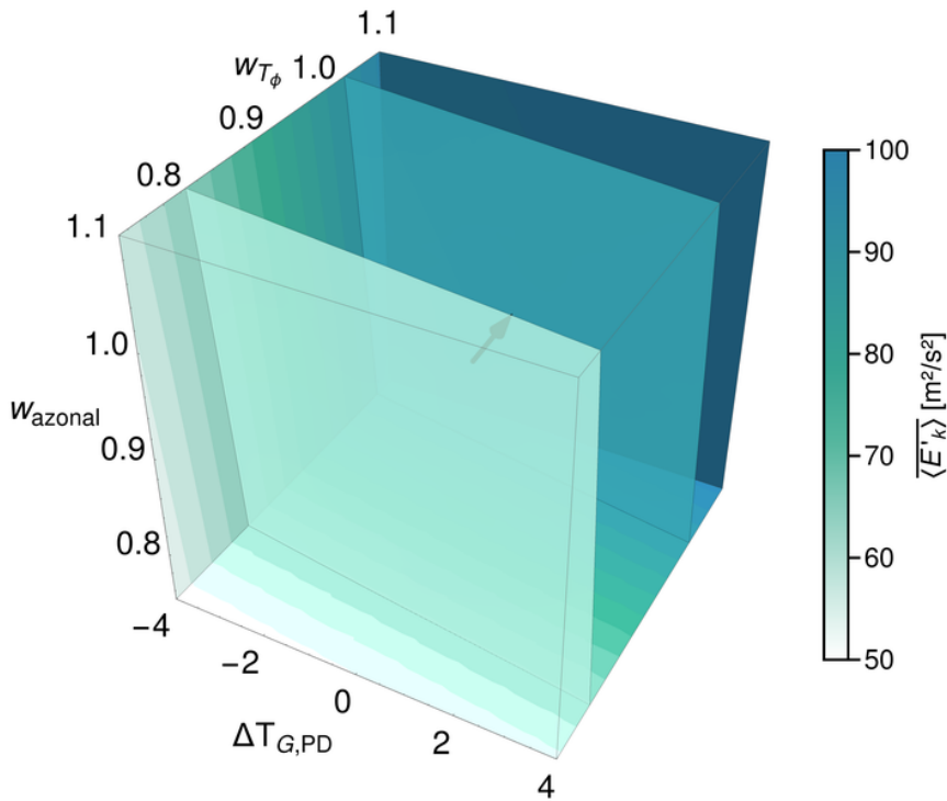
Fig. 8 Strength of the vertical integrated storm track activity in dependence of w_{T\phi} and w_{azonal} and \Delta T_{G,PD} . The arrow points in the direction of the strongest gradient.
