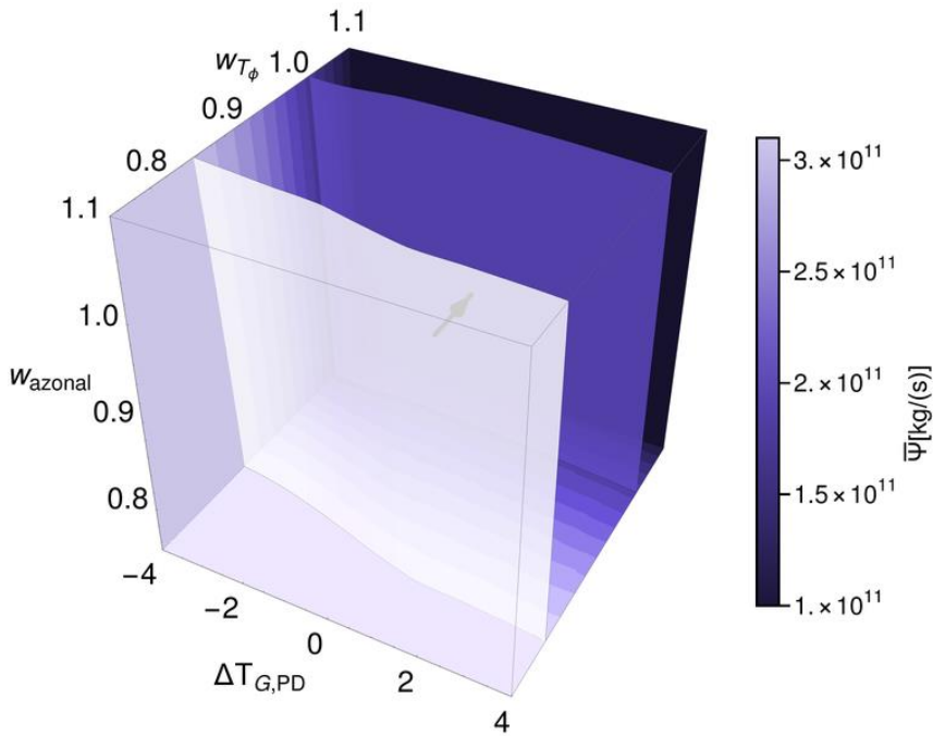
Fig. 4 Strength of the Hadley cell in dependence of w_{T\phi} and w_{\text{azonal}} and \Delta T_{G,PD} . The arrow points in the direction of the strongest gradient in boreal winter.
