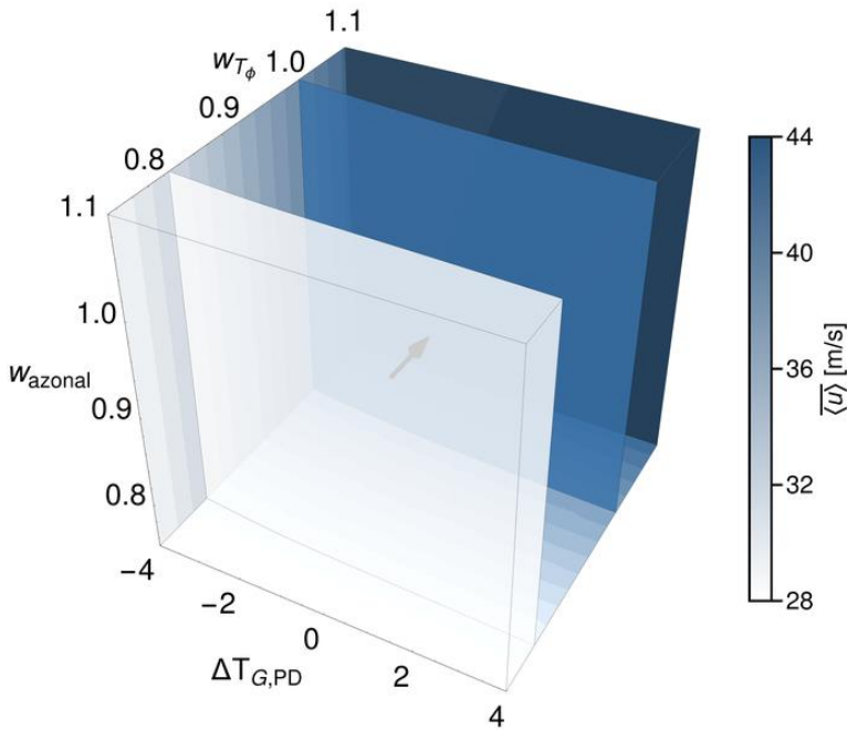
Fig. 6 Jet stream strength defined by the maximum of the zonal mean zonal wind velocity ( \langle \bar{u} \rangle ) between 10°N and 80°N at a height of 9000 m (corresponds to 300mb) in dependence of w_{T\phi} and w_{azonal} and \Delta T_{G,PD} in boreal winter.
