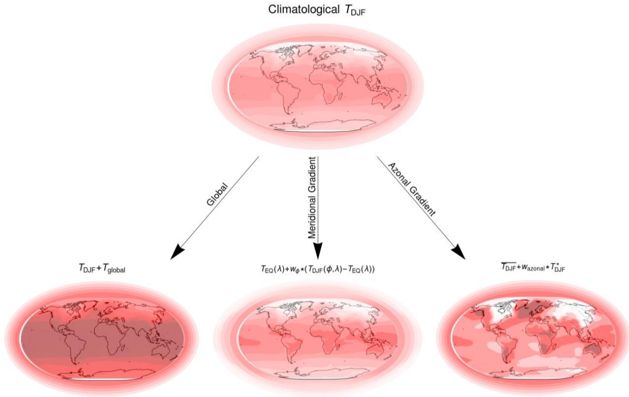
5 Fig. 1 Schematic illustration of the temperature perturbations.
