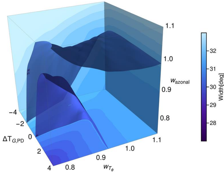
Fig. 3 Width of the Hadley cell in dependence of w_{T_\phi} and w_{azonal} and \Delta T_{G,PD} , whereby \Delta T_{G,PD} is the difference between the present day temperature and the altered global mean temperature in boreal winter.
