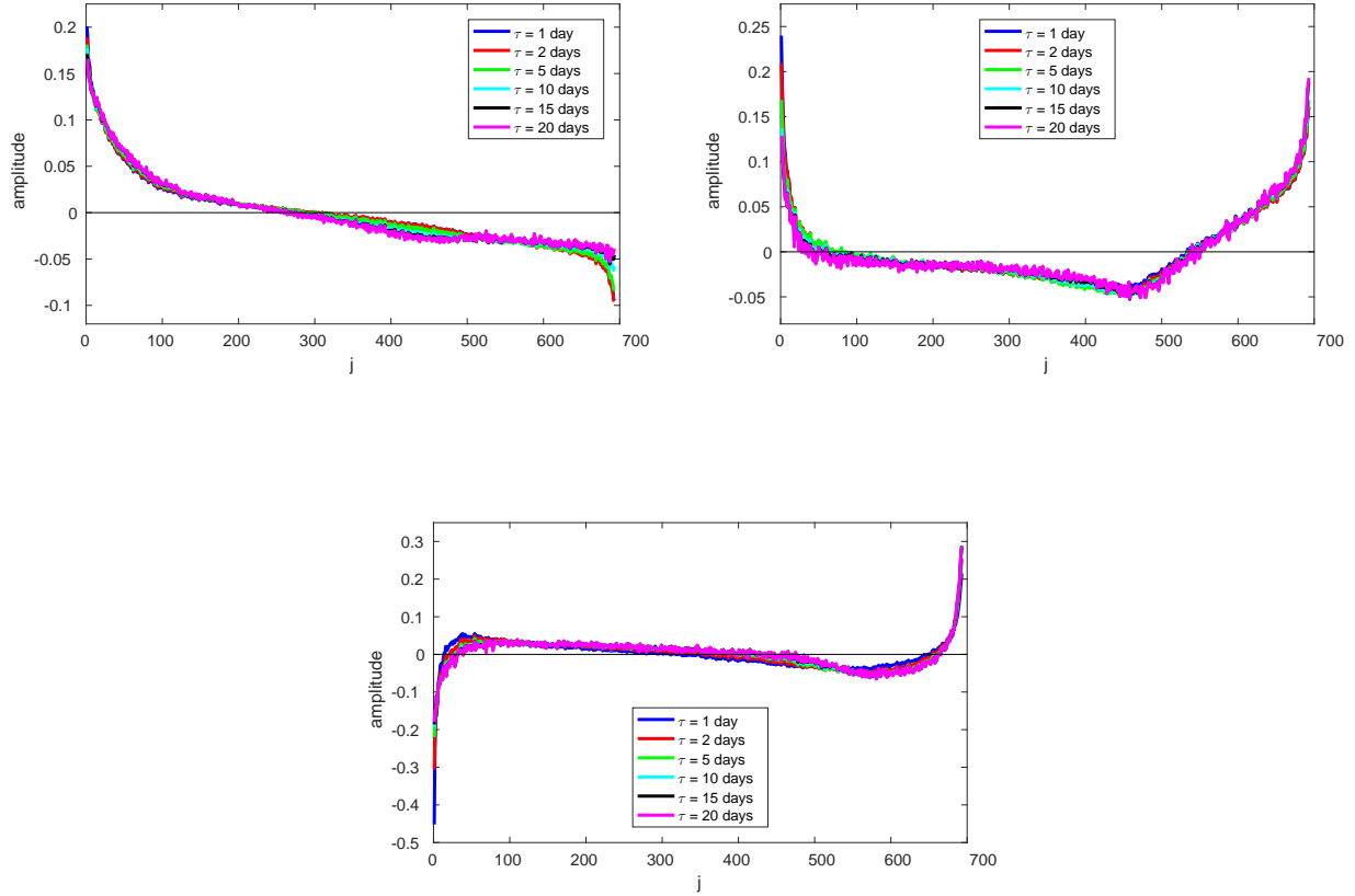
Figure 4. (a) First, (b) second and (c) third empirical orthogonal function (EOF) of the finite-time Lyapunov fluctuations.
