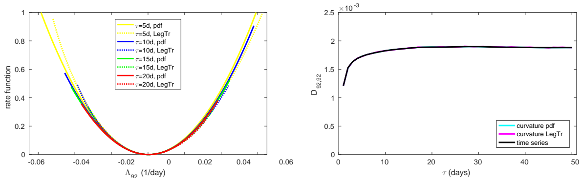
Figure 9. (a) Large-deviation rate function of the 92th FTLE. (b) Element D_{92,92} of the diffusion matrix.
