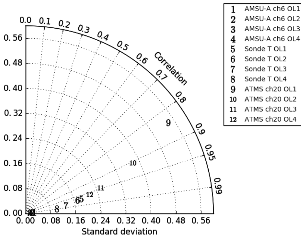
Figure 4. Taylor diagram showing the correlation (azimuthal angle) and standard deviation (distance from the origin) of differences in observation departures between nonlinear trajectory and linear minimisation steps for each outer loop for different observation types (ASMU-A channel 6, radiosonde temperature and ATMS channel 20).
