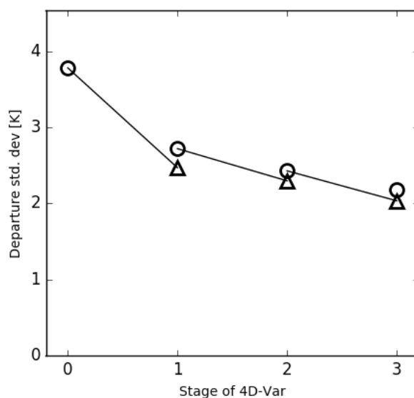
Figure 3. Standard deviation of departures for AMSR-2 channel 10 in the nonlinear trajectories (circles) and linear minimisation steps (triangles) for each outer loop of 4D-Var. Results from a single cycle from the ECMWF operational assimilation system.
