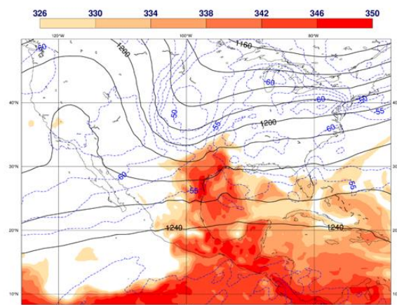
Figure 8. Left panel: Infrared image of the continental US from the GOES-13 geostationary satellite, valid on 2017-05-03 17.45 UTC (credits: National Centers for Environmental Information, NOAA). Right panel: ECMWF operational analysis of geopotential at 200 hPa (continuous isolines), temperature at 200 hPa (dashed isolines) and equivalent potential temperature at 850 hPa (shaded, units Kelvin), valid on 2017-05-03 18 UTC.
