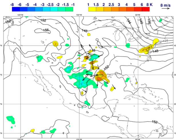
Figure 9 Left panel: ECMWF operational analysis of geopotential at 200 hPa (continuous isolines), temperature analysis increments at 150 hPa (colour shaded, units Kelvin) and wind vector analysis increments at 150 hPa (arrows, units m/s), valid on 2017-05-03 12 UTC. Right panel: as left, all quantities at 850 hPa.
