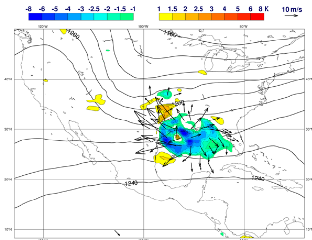
Figure 9 Left panel: ECMWF operational analysis of geopotential at 200 hPa (continuous isolines), temperature analysis increments at 150 hPa (colour shaded, units Kelvin) and wind vector analysis increments at 150 hPa (arrows, units m/s), valid on 2017-05-03 12 UTC. Right panel: as left, all quantities at 850 hPa.
