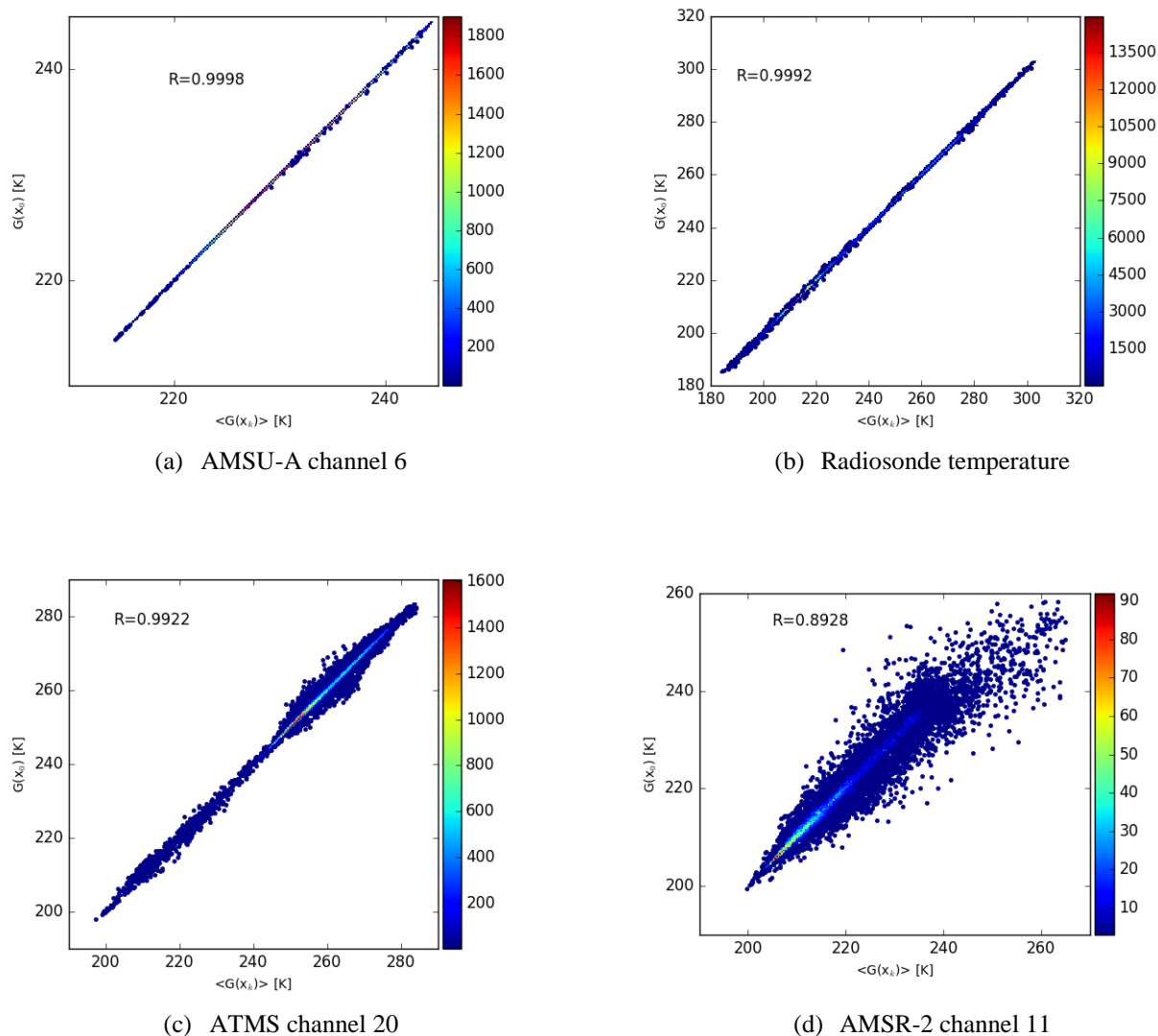
Figure 2. Ensemble mean G(x) (x-axis) against control member G(x) for (a) AMSU-A channel 6 in clear sky locations (b) radiosonde temperature (c) ATMS channel 20 (clear sky) and (d) ASMR-2 channel 11 observations (all-sky).
