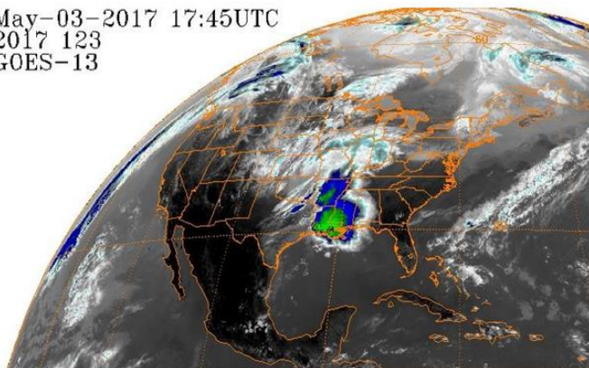
Figure 8. Left panel: Infrared image of the continental US from the GOES-13 geostationary satellite, valid on 2017-05-03 17.45 UTC (credits: National Centers for Environmental Information, NOAA). Right panel: ECMWF operational analysis of geopotential at 200 hPa (continuous isolines), temperature at 200 hPa (dashed isolines) and equivalent potential temperature at 850 hPa (shaded, units Kelvin), valid on 2017-05-03 18 UTC.
