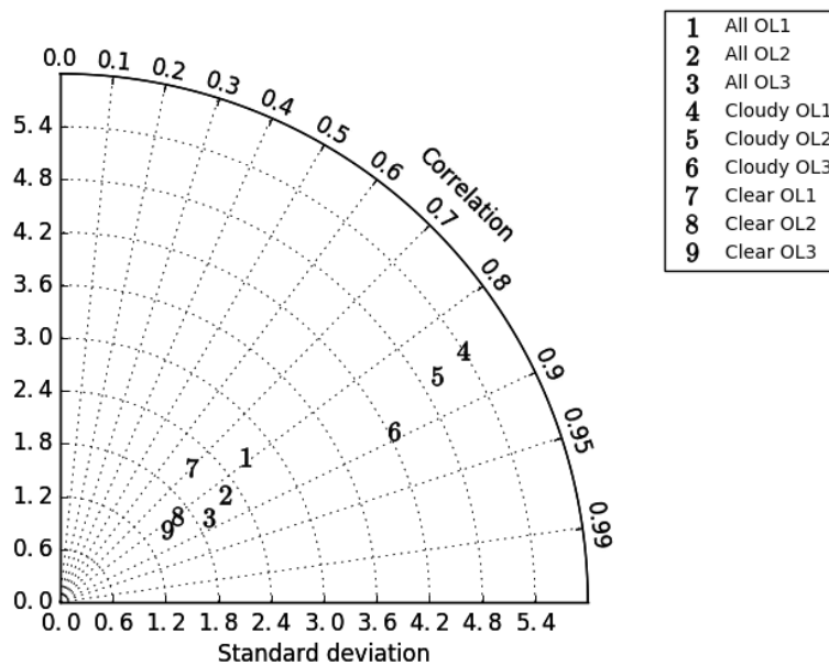
Figure 5. As Fig. 4 but showing results from AMSR-2 channel 11 categorising observations by those in clear sky regions and those impacted by cloud.
