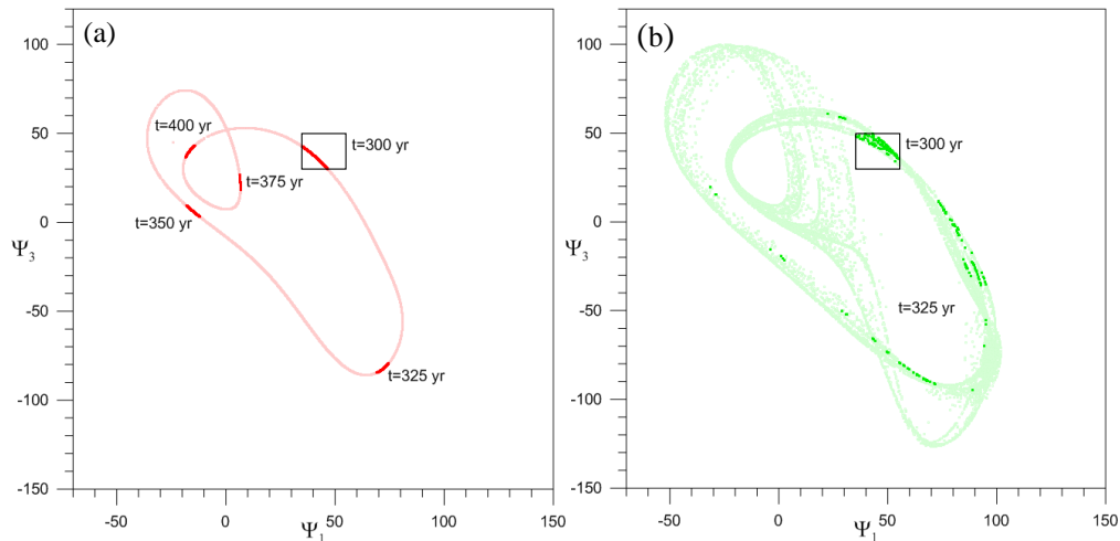
Figure 5. Chaotic and not non chaotic behavior of the autonomous model. (a) Evolution of the 1774 points (red dots) contained at t = 300 yr in the black rectangle of Fig. 4c for \gamma = 1.1 ; the attractor is illustrated by the entire set of 15 000 points, shown in light red. (b) Same but for the 135 points (green dots) that lie within the same rectangle for \gamma = 1.35 ; in this case, the attractor composed of the 15 000 points is shown in light green. Due to the chaotic nature of the dynamics in this case, only one snapshot, after 25 yr, is drawn.
