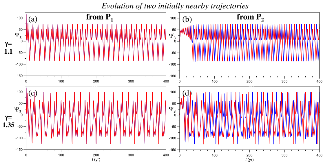
Figure 3. Typical behavior of time series evolution of \Psi_3(t) for different values of the parameter \gamma and different initial points in \Gamma . (a) Two trajectories obtained for \gamma = 1.1 and initialized at P_1 (red line) and at a nearby point (blue line). (b) Same as in panel (a), but for two trajectories starting from the point P_2 (red) and near it (blue). (c,d) Same as in (a,b) but for \gamma = 1.35 .
