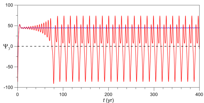
Figure 12. Fixed point P_0 of the autonomous case, with \varepsilon = 0 . Time series evolution of \Psi_3 for the trajectory initialized at P_0 = (-16, -83) (blue line) and at a nearby point (solid red line) for \gamma = 1.1 and T_p = 30 yr .
