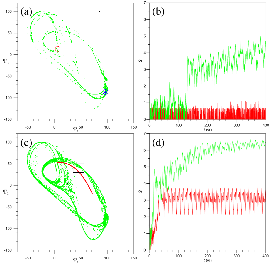
Figure 4. Chaotic and not non chaotic behavior of the autonomous model, for time-independent forcing intensity \gamma = 1.1 (red) and \gamma = 1.35 (green), respectively. Typical behavior of (a,c) the trajectories in the model's phase plane (\Psi_1, \Psi_3) ; and (b,d) of the model's entropy S_\theta(t) . (a) Intersection with the (\Psi_1, \Psi_3) -plane at t = 300 yr of 15 000 trajectories emanating from the small square box \vartheta_1 of width \Delta\Psi = 2 and centered at the point P_1 (black dot), for \gamma = 1.1 (red dots, enclosed in the red circle ) and for \gamma = 1.35 (green dots); for the blue dots see the text . (b) Time series evolution of the corresponding entropy S_{\vartheta_1} for \gamma = 1.1 (red line) and \gamma = 1.35 (green line). (c,d) Same as panels (a, eb ), but for the initial box \vartheta_2 centered at P_2 , likewise shown as a black dot in (c). For the evolution of the points contained at t = 300 yr in the black rectangle of panel (c), see Fig. 5 below.
