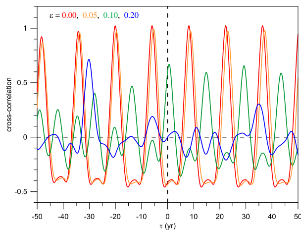
Figure 10. Cross-correlation c(\tau) between the two initially nearby trajectories shown in Figs. 9a–d, computed for the centered and normalized anomalies \tilde{\Psi}_3 , according to Eq. (7), for \varepsilon = 0 (red line), 0.05 (orange line), 0.1 (green line), and 0.2 (blue line).
