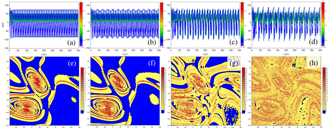
Figure 6. Transition from a periodic to a chaotic PBA as the amplitude \varepsilon of the periodic forcing in Eq. (3) increases. (a,b,c,d) Time series evolution of P_{\Psi_3} ; and (e,f,g,h) maps of \sigma for \gamma = 1.1 , T_p = 30 yr and \varepsilon = 0, 0.05, 0.1 , and 0.2 , respectively.
