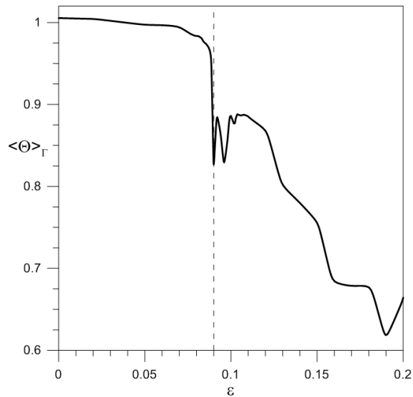
Figure 13. Transition from periodic to chaotic behavior, illustrated by the metric \langle \Theta \rangle_{\Gamma} , plotted vs. the amplitude \varepsilon of the periodic forcing in Eq. (3); \gamma = 1.1 and T_p = 30 yr.
