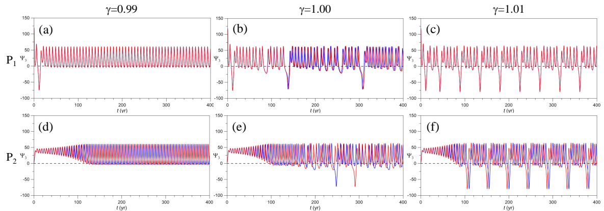
Figure 15. Critical transition in the autonomous system at \gamma_c . Panels (a,d), (b,e) and (c,f) correspond to \gamma = 0.99, 1.0 and 1.01 , respectively. (a,b,c) Time series evolution of \Psi_3 for the trajectory initialized at P_1 (red line) and at a nearby point (blue line); (d,e,f) same but for trajectories initialized at P_2 .
