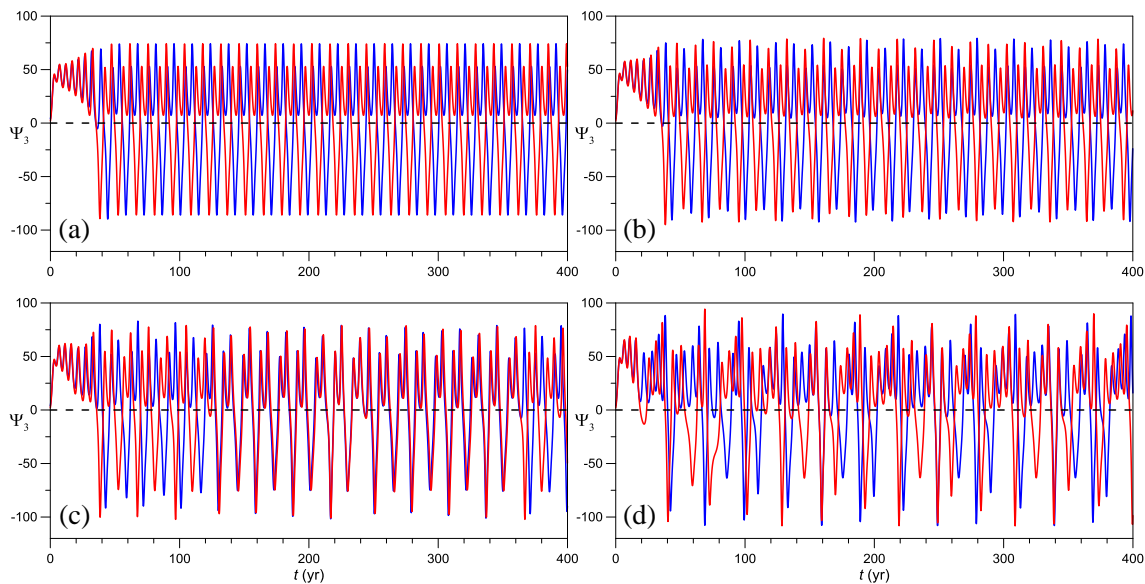
Figure 9. Increasing instability of trajectories as \varepsilon increases. Time series evolution of \Psi_3(t) for the trajectory initialized at the point P_2 (red line) and at a nearby point (blue line) for \gamma = 1.1, T_p = 30 yr, and (a–d) \varepsilon = 0, 0.05, 0.1 , and 0.2 .
