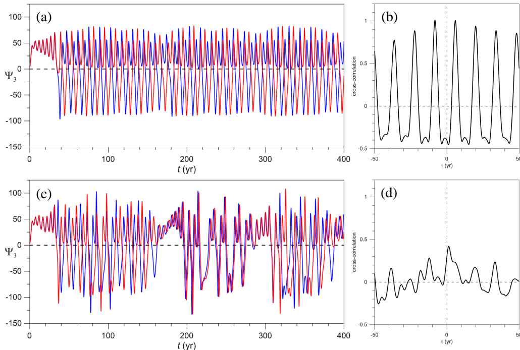
Figure 18. Role of the cross-correlation diagnostics in characterizing chaotic behavior for an aperiodically forced system, given by Eqs. (2) and (11); \gamma = 1.1 . (a) Time series evolution of \Psi_3 for \varepsilon' = 0.05 in Eq. (11); and (b) corresponding cross-correlation. (c,d) Same as (a,b) but for \varepsilon' = 0.2 . The trajectories initialized at P_2 are in red and those initialized at a nearby point are in blue.
