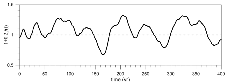
Figure 17. Aperiodic forcing G(t)/\gamma of the idealized ocean model as— defined in—by Eq. (11) herein, with—and plotted using the value \varepsilon' = 0.2 , as adopted in Pierini et al. (2016).
