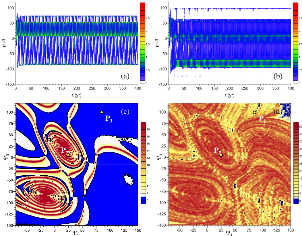
Figure 2. Distinct autonomous regime behavior for (a,c) \gamma = 1.1 , and (b,d) for \gamma = 1.35 . Upper panels: time series evolution of P_{\Psi_3} for (a) \gamma = 1.1 , and (b) \gamma = 1.35 . Lower panels: maps of the mean normalized distance \sigma for (c) \gamma = 1.1 , and (d) for \gamma = 1.35 ; the points P_1 = (85, 100) and P_2 = (25, 5) appear in the panels (c) and (d), respectively. Note the different scales in the two maps; 15 000 trajectories, with regularly spaced initial points in \Gamma , were used for both maps.
