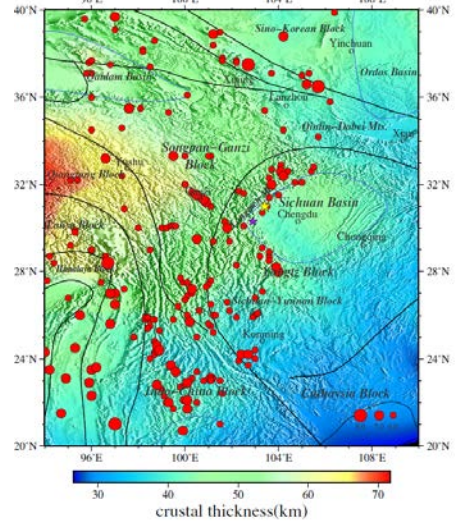
Figure 7. Crustal thickness of model CUB2 from Shapiro & Ritzwoller (2002). Note: Color scale is not exactly the same with figure 6.
