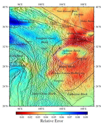
Figure 9. The relative error of the average phase velocity between the phase velocity calculated by our model and the phase velocity observed by Xie (2013).
