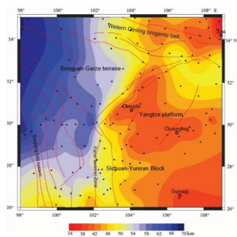
Figure 10. Contour map of crustal thickness estimated by h-k stacking analysis based on the receiver function(Wang ,2010, Small black solid circles indicate seismic station used by wang(2010)).
