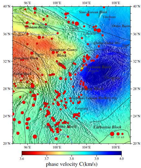
Figure 4. Average phase velocity of western Yangtze craton(Xie et al.,2013) from 10 to 35mHz.The black lines in the figure show structure lines. The blue lines show boundaries of sedimentary basins. The red dots show seismic events in this region from 1975 to 2015, and size of dot demonstrates size of magnitude from Ms 6.0 to Ms 8.0. The yellow and purple stars demonstrate Wenchuan and Lushan earthquakes respectively. These are same to Figure 4, Figure 6 and Figure 7.
