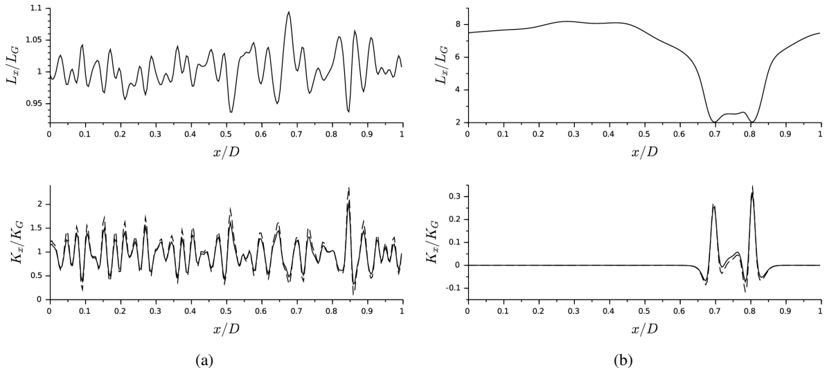
Figure 3. Diagnoses of the length-scale normalized by L_G (top panels) and of the kurtosis (normalized by K_G = \frac{1}{8}g_G^2 ) deduced from the ensemble of forecast with initial uncertainty magnitude \sigma_{10\%}^0 , at times t = 0 (a) and t = T (b) (continuous line). The kurtosis is compared with its closure K_x^{GC} = \frac{1}{8}g_x^2 - \frac{1}{12}\partial_x^2 g_x (dashed line) computed from the metric field.
