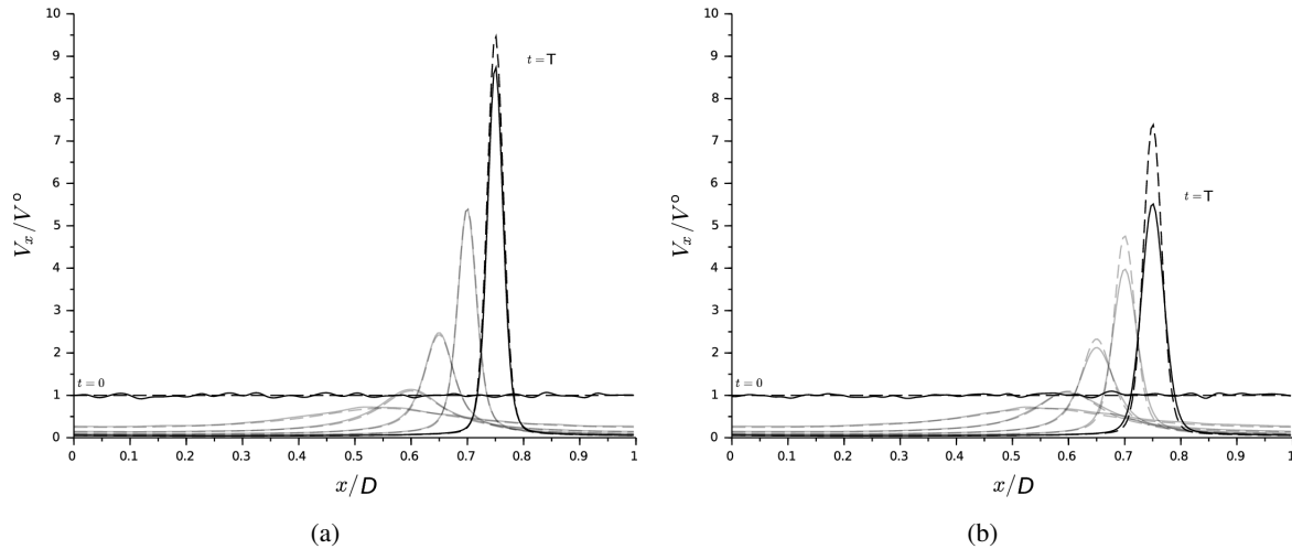
Figure 4. Analytical (dashed line) versus numerical (continuous line) variance fields for initial perturbation of standard deviation magnitude \sigma_{1\%}^0 (a) (tangent-linear dynamics) and \sigma_{10\%}^0 (b) (weakly nonlinear dynamics). The fields are represented only for the times t = \{0, 0.2, 0.4, 0.6, 1\}T .
