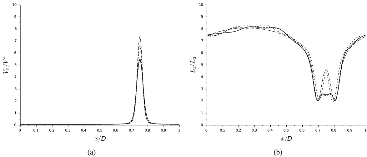
Figure 6. Verification of the theoretical variance (a) and correlation length-scale (b) at t = T and for an initial perturbation standard deviation \sigma_{10\%}^0 . The results for the nonlinear ensemble are in continuous line, the theoretical statistics are in dashed line, the ensemble without (with) second order term \varepsilon \partial_x \varepsilon is in small dashed line (dash-dotted line), respectively.
