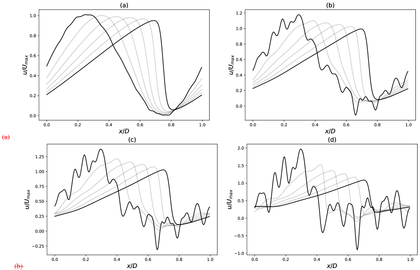
Figure 2. Solutions from the initial perturbations of magnitude (a) \sigma_{1\%}^0 and (b) \sigma_{10\%}^0 , (c) \sigma_{20\%}^0 and (d) \sigma_{50\%}^0 , for the times t = \{0, 0.2, 0.4, 0.6, 1\}T and t = \{0, 0.2, 0.4, 0.6, 0.8, 1\}T .
