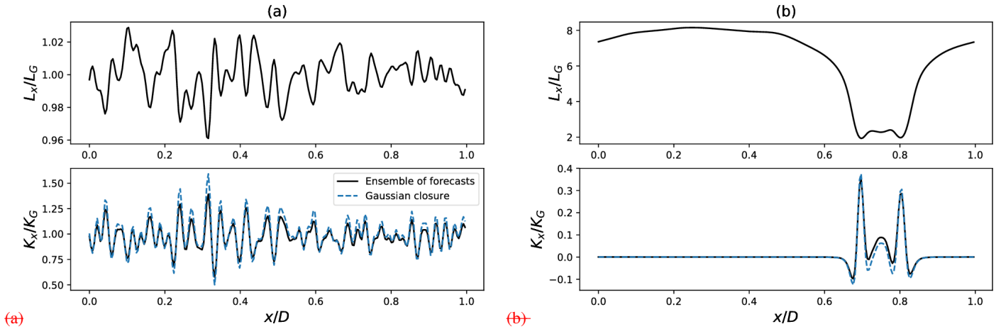
Figure 3. Diagnoses of the length-scale L_x normalized by L_G L_G (top panels) and of the kurtosis (normalized by K_G = \frac{1}{8}g_G^2 , K_G = \frac{1}{8}g_G^2 ) (bottom panels) deduced from the ensemble of forecast with initial uncertainty magnitude \sigma_{10\%}^0 , at times t = 0 (a) and t = T (b) (continuous line). The kurtosis is compared with the its closure K_x^{GC} = \frac{1}{8}g_x^2 - \frac{1}{12}\partial_x^2 g_x , K_x^{GC} = \frac{1}{8}g_x^2 - \frac{1}{12}\partial_x^2 g_x (dashed line) computed from the metric field.
