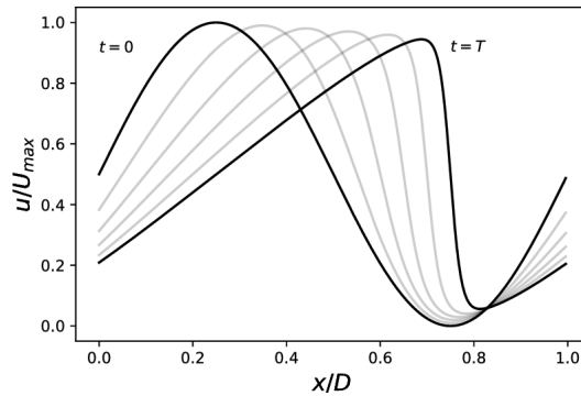
Figure 1. Nonlinear solution of the diffusive Burger' equation for the times t = \{0, 0.2, 0.4, 0.6, 1\}T t = \{0, 0.2, 0.4, 0.6, 0.8, 1\}T .
