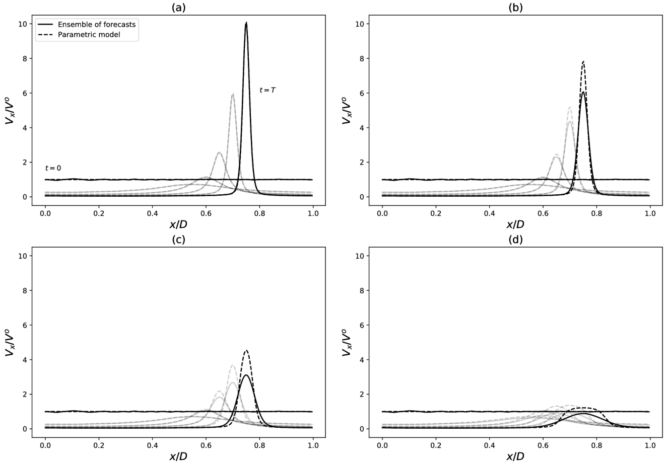
Figure 5. Parametric (dashed line) versus ensemble estimated (continuous line) variance fields for initial perturbations of standard deviation magnitude \sigma_1^0\% (a) (tangent-linear dynamics), \sigma_{10}^0\% (b) (weakly nonlinear dynamics), \sigma_{20}^0\% (c) and \sigma_{50}^0\% (d). The fields are represented only for the times t = \{0, 0.2, 0.4, 0.6, 0.8, 1\}T .
