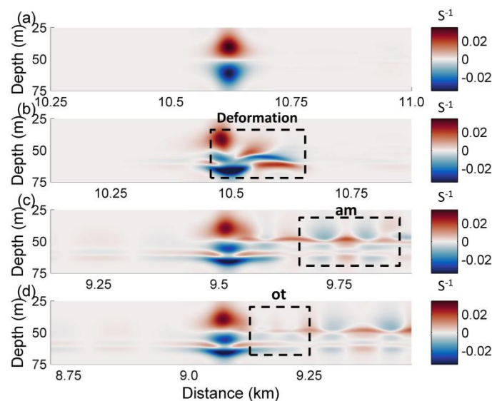
5 Figure 8. The evolution process of the vorticity field in the case O9 ( \Delta = 0 ) for the different times (a) 0T, (b) 1.2T, (c) 10T, (d) 14T, where ‘am’ and ‘ot’ denote the amplitude-modulated wave packet and oscillating tail, respectively.
