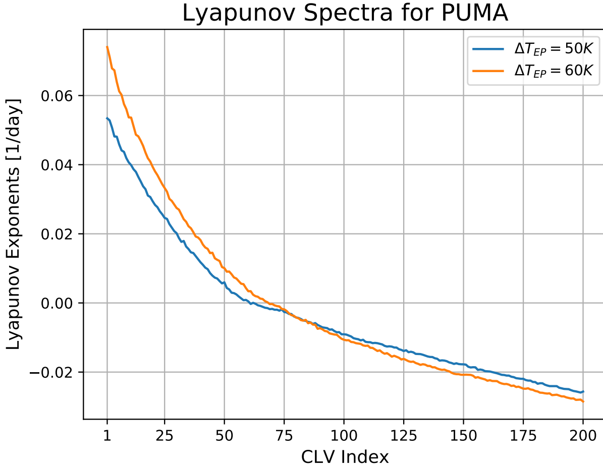
Figure 1. The 200 largest LEs of the Lyapunov spectra of PUMA for the two different setups with \Delta T_{EP} = 50K and 60K .
