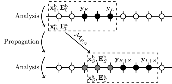
Figure 2. Chaining of the 4D-Var and IEnKS two first cycles with S = 3, L = 4 . The first 4D-Var analysis use the background \mathbf{x}_0^b at t_0 and the observations \mathbf{y}_{L:K} to produce the analysis \mathbf{x}_0^a at t_0 . It is propagated S steps forward in time to produce the new background at time t_S where another analysis can be performed. The IEnKS does the same but with an ensemble. The dashed rectangle symbolizes the current DAW, black dots represent the observations assimilated in the current cycle, gray dots represent already assimilated observations and white dots represent observations not assimilated.
