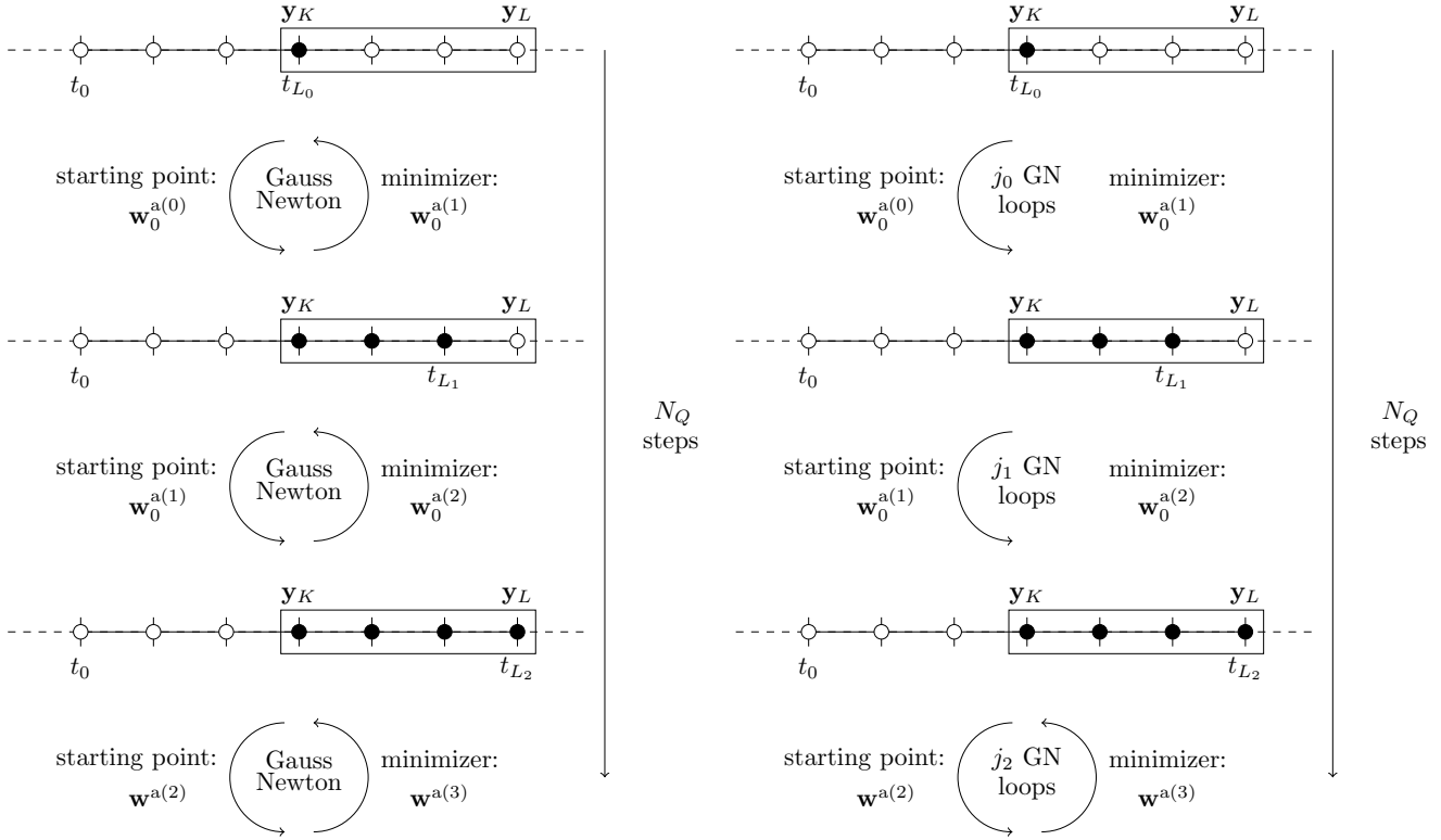
Figure 7. Schematics of an IEnKS-QS minimization (on the left) and an IEnKS-QC minimization (on the right). The rectangle contains the observations to be assimilated, the black dots represent the observations used in the current minimization. The "Gauss-Newton" surrounded by arrows represents the iterations of the Gauss-Newton procedure. The number of quasi-static steps is N_Q = 3 . The flow of observations is controlled by the parameters (L_0, L_1, L_2) = (3, 5, 6) . For the QC IEnKS, the number of GN iterations is controlled by the (j_0, j_1, j_2) parameters.
