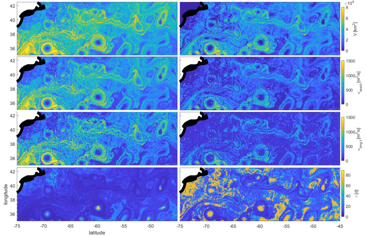
Figure 4. (will add 4 right panels corresponding to eddy-induced estimates) Encounter number (1 st row), exact diffusivity (2 nd row), long-time diffusivity (3 rd row) and diffusive time-scale (4 th row) for the full flow (left) and for the eddy component of the flow (right). The encounter volume was computed on 11/01/2015 over 90 days with a radius of 3°. The lower panel shows comparison between numerically-computed V and the long-time diffusive formula (38) with the corresponding \kappa for the 3 reference trajectories located in the core, periphery and outside (blue, magenta, green) of the Gulf Stream ring.
