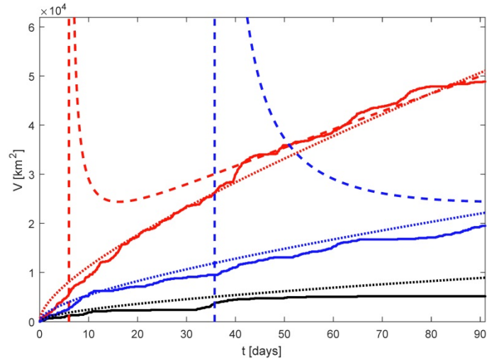
Figure 5. Comparison between numerically-computed V (solid) and the exact (dotted) and long-time diffusive formulas (dashed) with the corresponding \kappa for the 3 reference trajectories located in the core, periphery and outside (black, red, blue) of the Gulf Stream ring.
