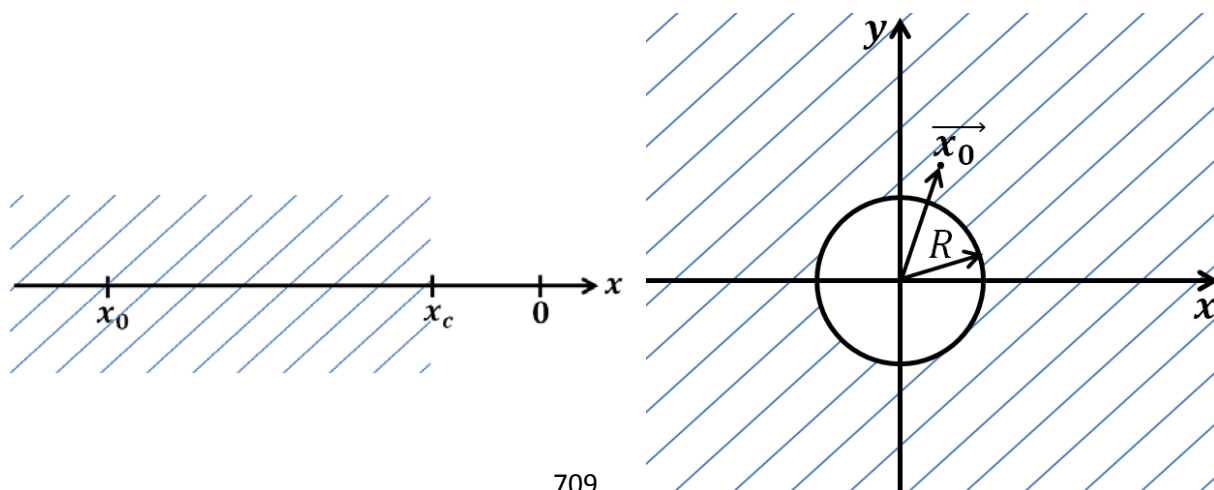
Figure 2. Schematic diagram in 1D (left) and 2D (right). Hatched areas show semi-infinite domains outside of the cliff.
