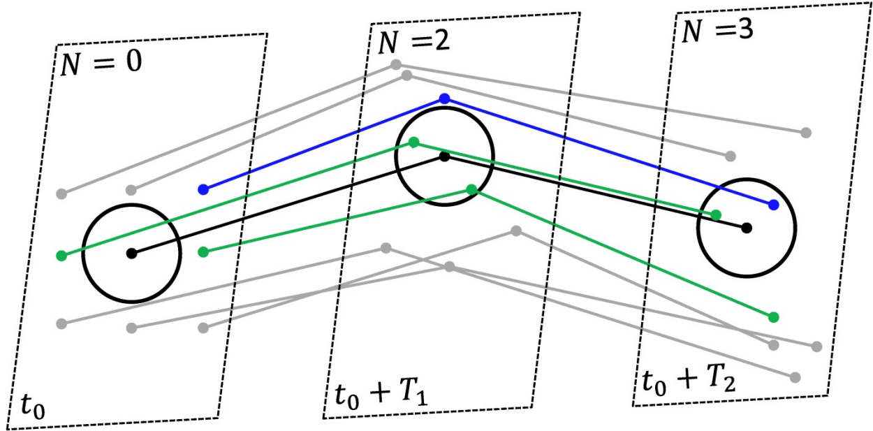
Fig. 1. Schematic diagram of trajectory encounters, showing trajectories of 9 particles, with dots indicating positions of particles at 3 time instances, at the release time, t_0 , and at two later times, t_0 + T_1 and t_0 + T_2 . The reference trajectory and the encounter sphere are shown in black, trajectories that do not encounter the reference trajectory are in grey, and trajectories that encounter the reference trajectory are in green if the encounter occur at t_0 + T_1 , and in blue if encounters occur at t_0 + T_2 . Time slices are schematically shown by dashed rectangles, and the encounter number, N , is indicated at the top of each time slice.
