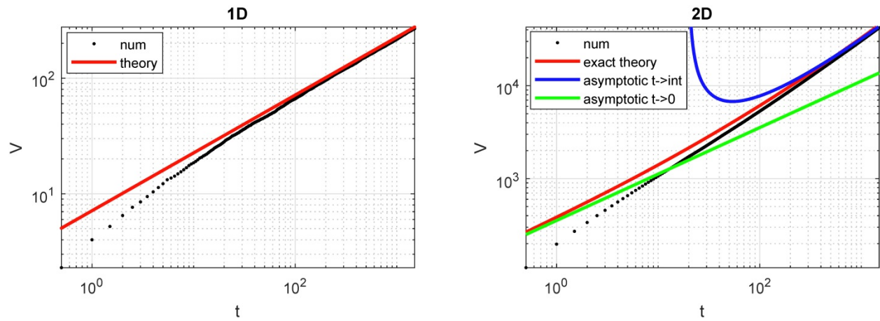
Figure 3. Comparison between theoretical expression (red, green, blue) and numerical estimates (black) of the encounter volume for a random walk in 1D (left) and 2D (right). In both, \kappa = 5 and \Delta t = 0.5 . In 2D, \tau \cong 20 .
