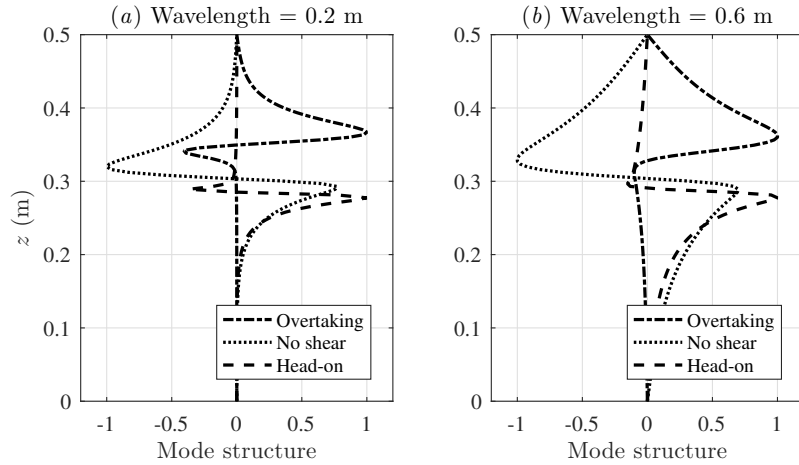
Figure 9. Same as figure 7 but for mode-2 waves.
