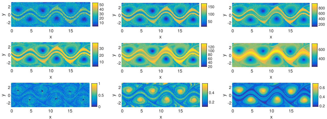
Figure 1. Network measures for high resolution initial conditions (case (i)) in the Bickley jet for \epsilon = 0.1 (left) and \epsilon = 0.2 (right middle) and \epsilon = 0.5 . From top to bottom: node degrees d and \langle d \rangle_{nn} and clustering coefficient C .
