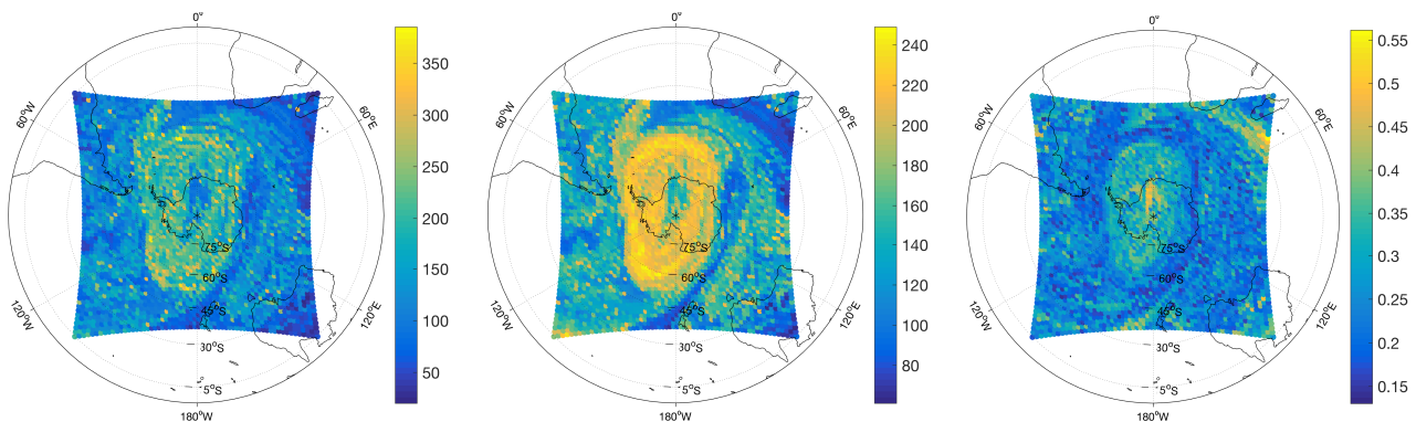
Figure 7. Average Node degree d (left), average node degree of neighboring nodes \langle d \rangle_{nn} (middle) and clustering coefficient C of a network constructed from trajectories for the polar vortex flow between September 1 and October 31, 2002. Left: particles at September 1, 2002; middle: September 26, 2002; right: October 31, 2002.
