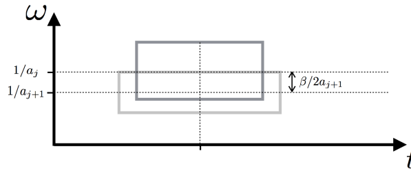
Figure C2. Example of rule for the discretization of scales taking into account the geometry of the uncertainty boxes. \beta = 1/\sqrt{2}\omega_0 > 0 .
