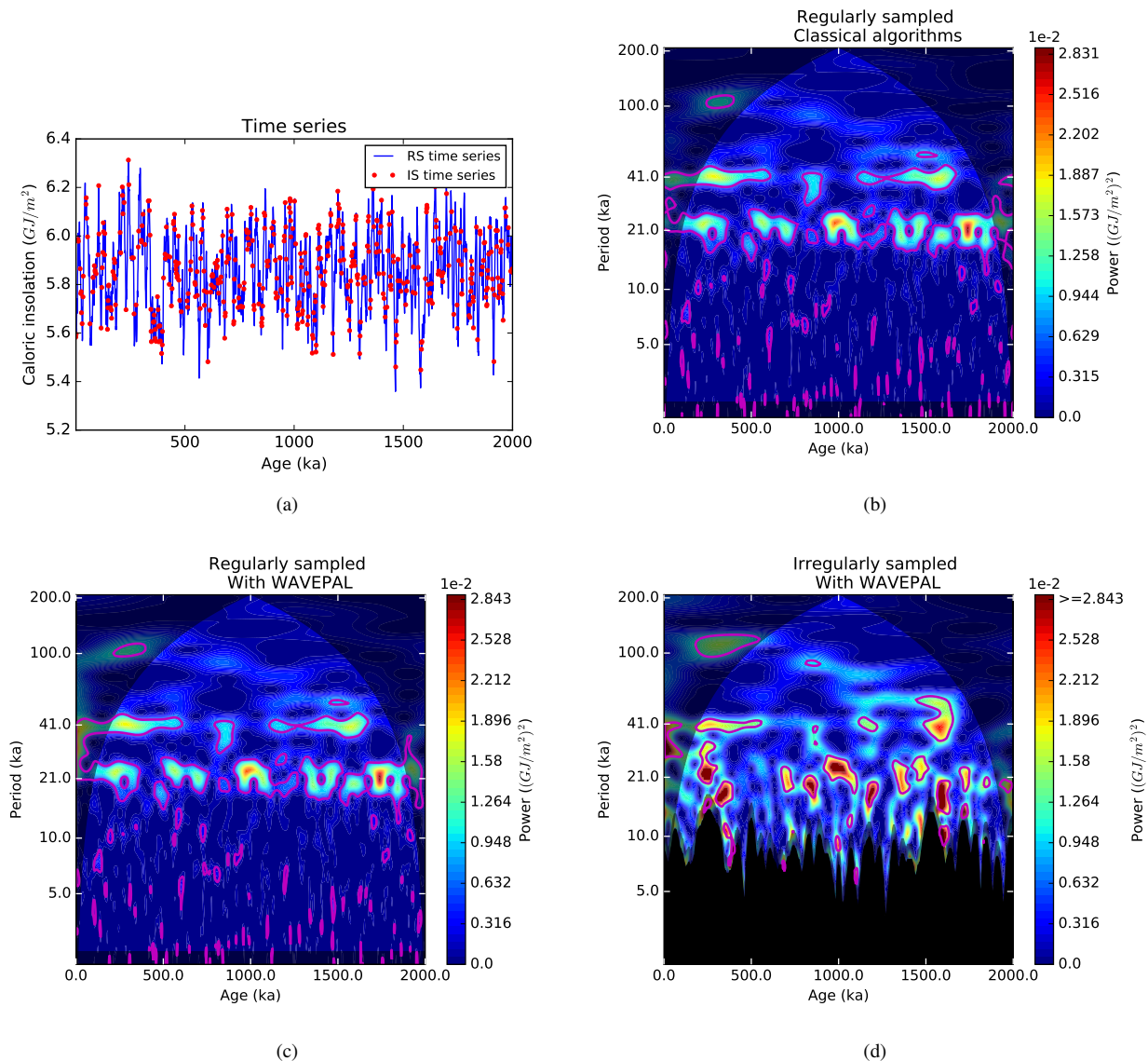
Figure 1. (a) The regularly sampled (RS) time series, with \Delta t = 1 ka, which represents the caloric summer insolation at 65^\circ N to which is added a realization of a Gaussian red noise process with \alpha = 0.1 and \sigma equal to half of the standard deviation of the original time series (these parameters are defined in Sect. 3.2.3 of paper I). The red dots are obtained from randomly removing 75% of the data points of the RS time series, resulting in an irregularly sampled (IS) time series with 500 data points. (b), (c) and (d) compare of the scalograms with \omega_0 = 10 , jointly with their 95% analytical confidence levels against a red noise background. (b) Scalogram of the RS time series computed with the classical approach. (c) Scalogram of the RS time series computed with WAVEPAL. (d) Scalogram of the IS time series computed with WAVEPAL. The black zone, called Shannon-Nyquist exclusion zone (SNEZ) and defined in Sect. 3.8, is the area where the sampling is not sufficient to probe the lowest periods. In (b), (c) and (d), the two lateral shaded areas are the half-cones of influence (see Sect. 3.7), and the bottom shaded area is the refinement of the SNEZ (defined in Sect. 3.10). The bounds of the color scale in the panels (b), (c) and (d) are the extrema of the scalogram in (c) over the non-shaded area, in order to make a meaningful visual comparison. Technical details about the computation of the scalogram and its confidence levels are given in Sect. 3 and 4.
