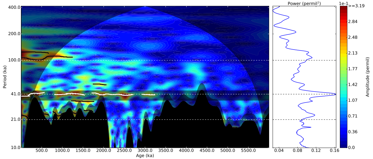
Wavelet amplitude - w_0=15
