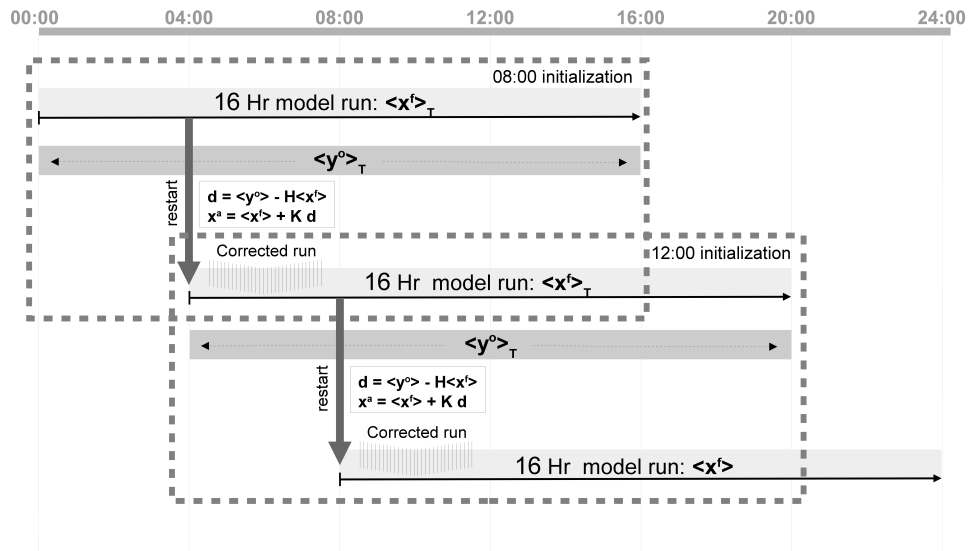
Figure 11. Data assimilation cycle in Oke et al. (2002). The time-distributed averaging procedure approach used to initialize the problem at time T/2 uses all the observations in the period [0, T] . In their application, the time T is approximately the inertial period.
