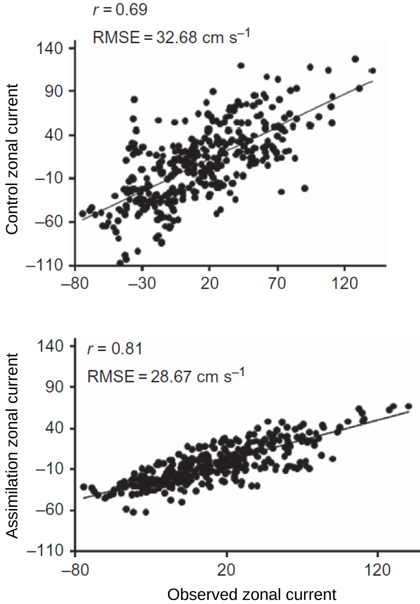
Figure 9. Correspondence between the zonal velocity component measured at the RAMA station located at 1.5^\circ \text{ N } 90.0^\circ \text{ E} . Upper plot model without assimilation. Lower plot, resulting from assimilating OSCAR currents. From figure 1 in Santoki et al. (2013).
