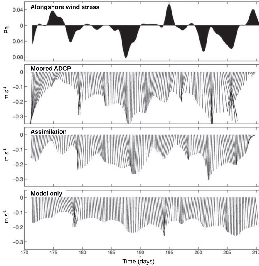
Figure 12. Comparison between the alongshore wind stress and the ocean vertical averaged current during the 40-day experiment. From figure 10 in Oke et al. (2002).
