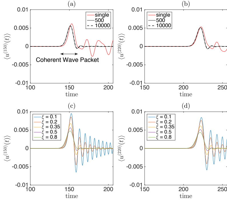
Figure 6. Displacements of 150^{\text{th}} - 150^{\text{th}} (Fig. 5(a) and Fig. 5(c)) and 220^{\text{th}} - 220^{\text{th}} (Fig. 5(b) and Fig. 5(d)) particle with respect to time for different ensembles (Fig. 5(a) and Fig. 5(b)) of disorder, \xi = 0.5 and of multiple disorder parameters (Fig. 5(c) and Fig. 6(d); for 500 ensembles).
