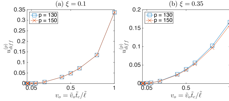
Figure 4. The nonlinear increase in u_{diff}^{(p)} (a parameter which shows dissimilarity between linear and nonlinear space time responses) with initial impulse velocity ( v_o ). The value v_o = 0.05 is in the zone where linear and nonlinear space time responses are almost identical.
