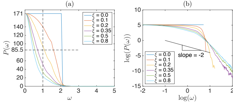
Figure 11. Participation Ratio or the Localization-length with respect to different frequencies for 500 ensembles with \xi = 0.1, 0.2, 0.35, 0.5 and 0.8 and bin size = 0.0781.
