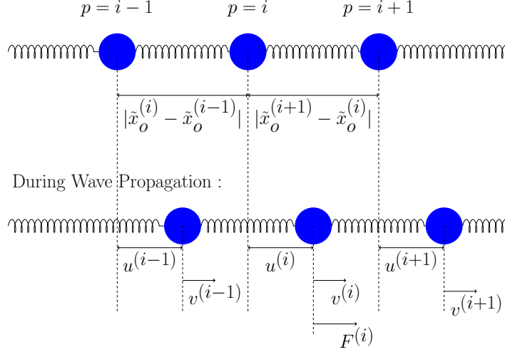
Figure 2. Chain Pre-stressed chain of granular elements during dynamic wave propagation with length scaled by the characteristic equilibrium distance \tilde{\Delta}_o .
