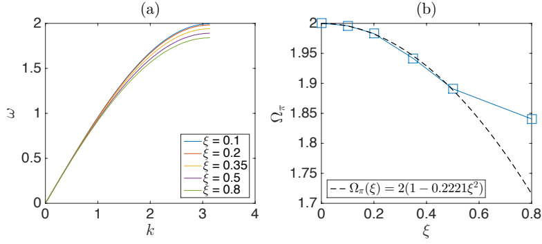
Figure 10. Dispersion relation (Fig. 10(a), \langle\Omega(k)\rangle ) with respect to different wavenumbers and (b) the maximum permissible frequency has been shown for disorder parameters, \xi = 0.1, 0.2, 0.35, 0.5 and 0.8 , with empirical quadratic fit given in the inset (ignoring \xi = 0.8 ).
