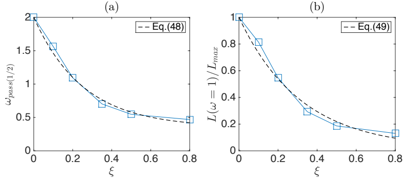
Figure 12. (a) \omega_{pass(1/2)} for different \xi and (b) Localization length at \omega = 1 scaled with maximum localization length ( L_{max} ) for different \xi .
